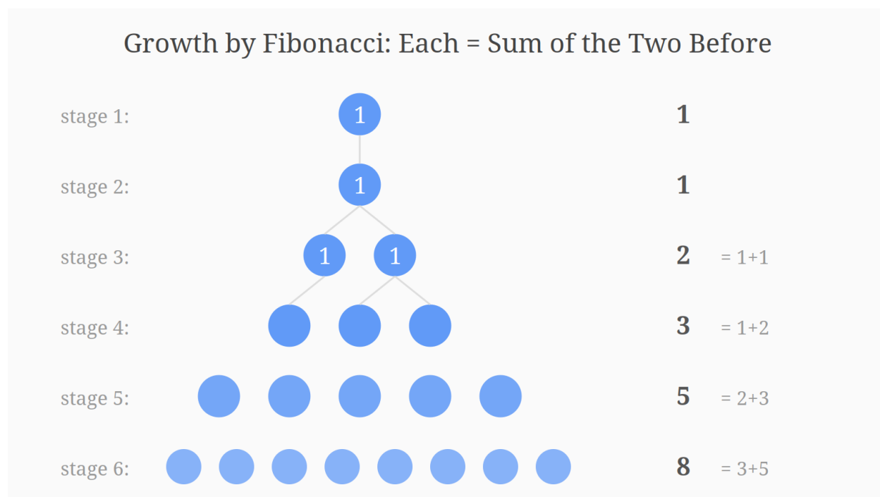
Figure 3: Fibonacci growth: each stage is the sum of the two before
