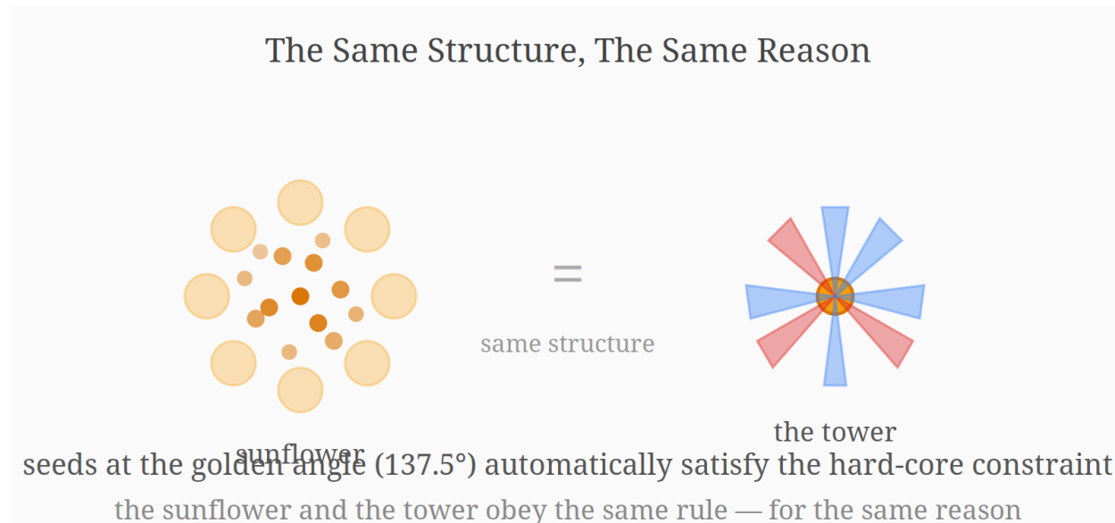
Figure 5: The same structure, the same reason — sunflowers and the tower obey one rule
