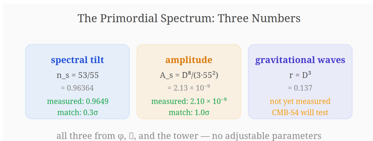
Figure 28: The primordial spectrum: three numbers from the tower
