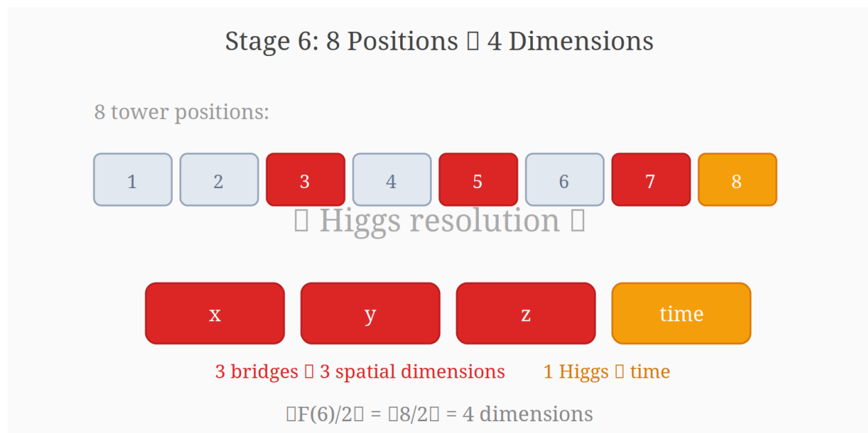
Figure 18: Stage 6: 8 positions resolve into 4 dimensions
