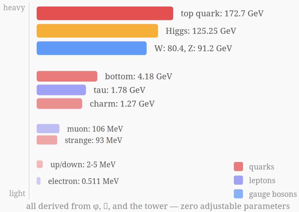
Figure 23: The mass ladder: every rung from the same ratio
