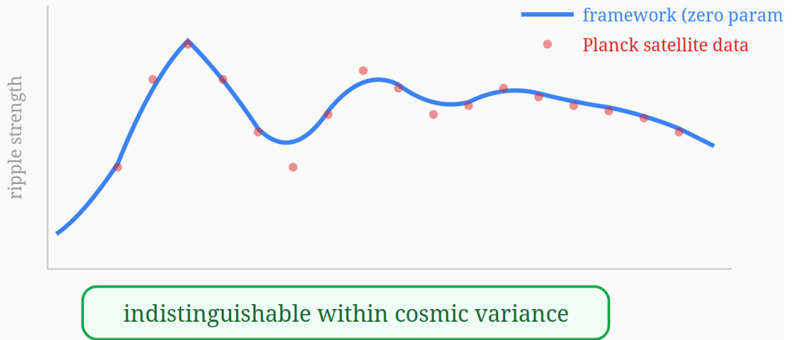
Figure 36: The hardest test: 2,500 data points, zero knobs
