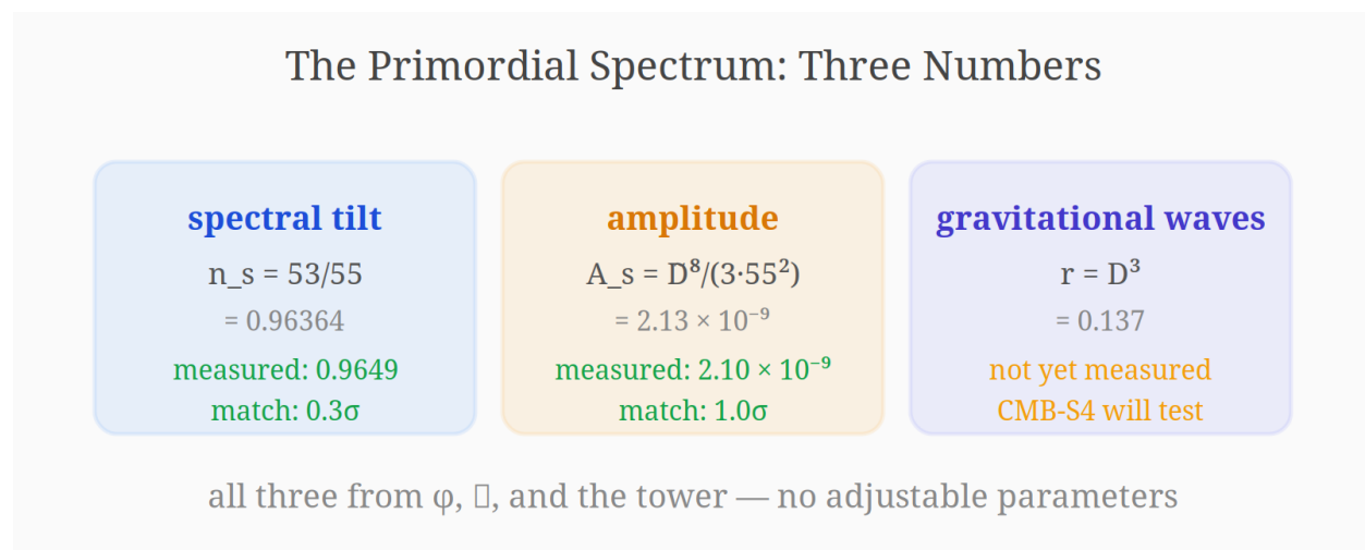
Figure 28: The primordial spectrum: three numbers from the tower
