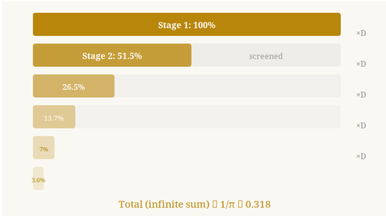
Figure 4: The Screening Tower: each layer dims by D
