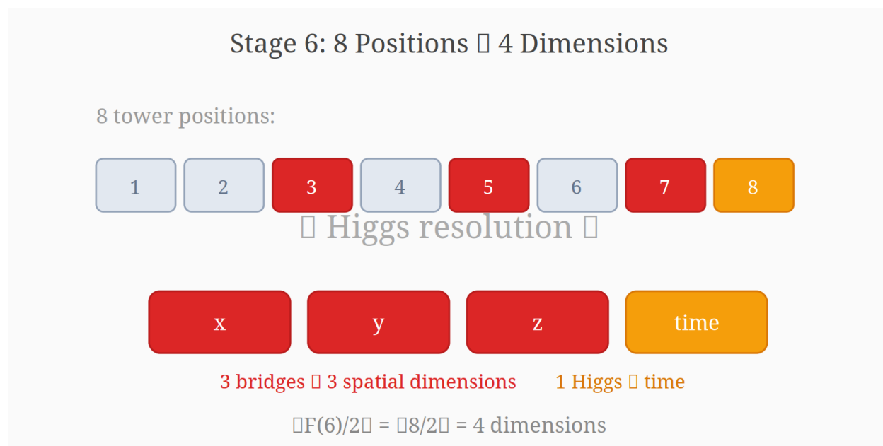
Figure 21: Stage 6: 8 positions resolve into 4 dimensions
