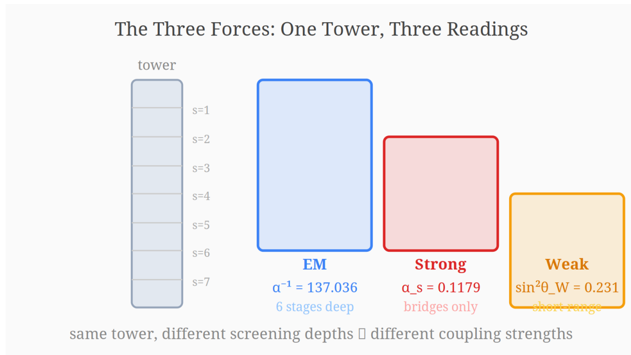
Figure 22: The three forces: one tower, three screening depths
