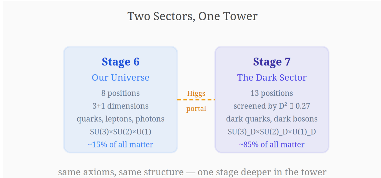
Figure 26: Two sectors, one tower: visible at stage 6, dark at stage 7
