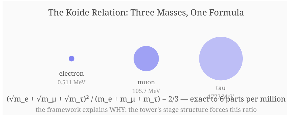
Figure 24: The Koide relation: three masses, one formula
