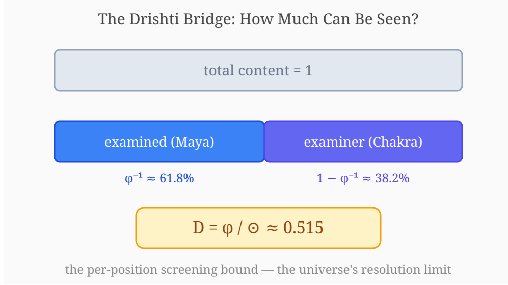
Figure 15: The Drishti Bridge: the observation bound D = \varphi/\pi
