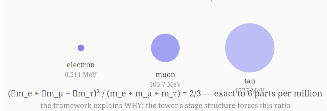
Figure 24: The Koide relation: three masses, one formula
