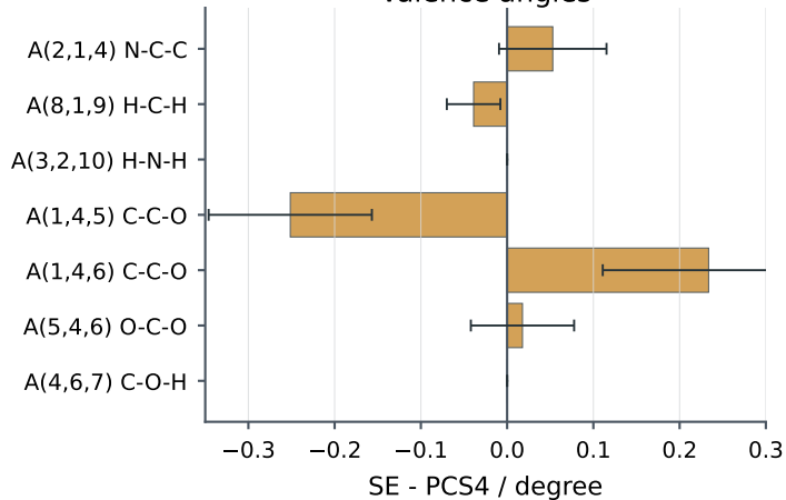
Valence angles
