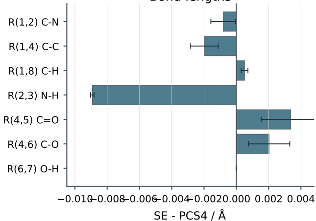
Bond lengths
