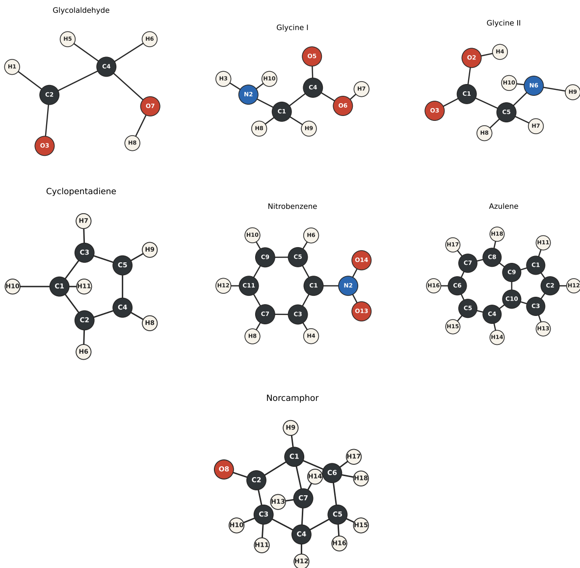
Figure 2: Atom numbering used for the glycolaldehyde, glycine I, glycine II, cyclopentadiene, nitrobenzene, azulene, and norcamphor semiexperimental refinements. The labels are derived from the Cartesian input order and are used consistently in the GIC definitions, primitive-coordinate constraints, and structural tables.
