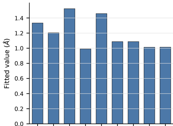
Bond lengths
