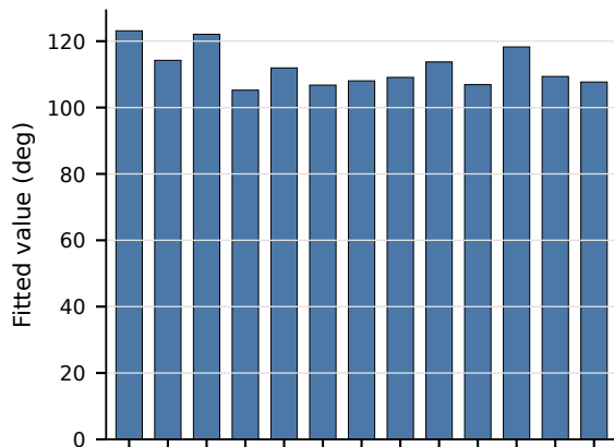
Valence angles
