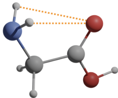
bifurcated \text{NH}_2 \cdots \text{O} motif
