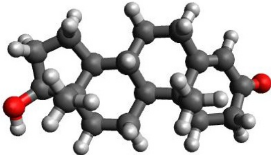
FIG. 9. Testosterone large-molecule scale demonstration. The 49-atom fused-ring molecule tests the complete path from a QC reference geometry and vibrational corrections to automated non-redundant coordinate generation and reduced structural models.
