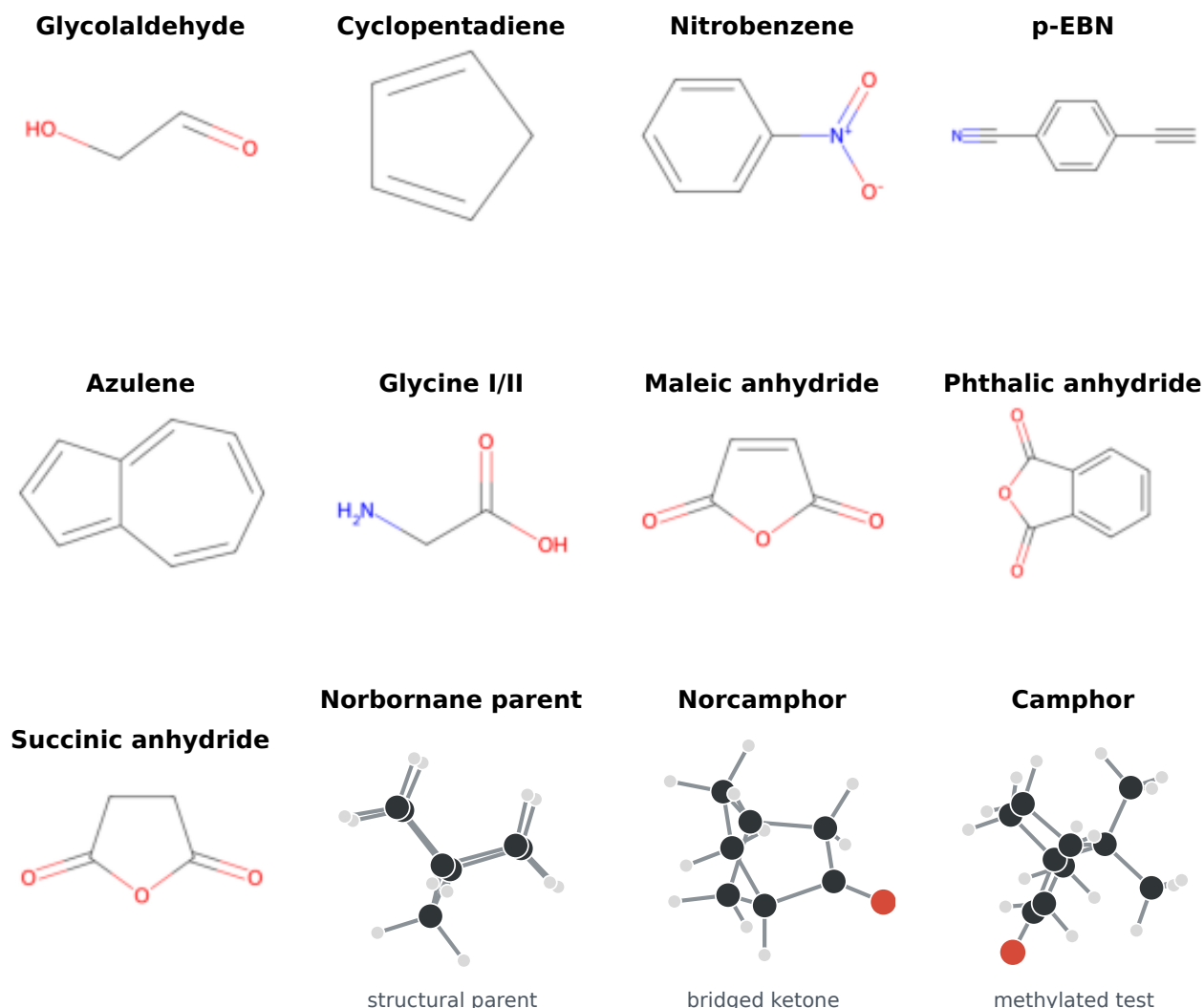
FIG. 2. Molecular structures used to test automated model construction. The acyclic, planar, aromatic, glycine, and anhydride benchmarks are shown as connectivity diagrams; the bridged norbornane family is shown as three-dimensional structures because its graph topology is not communicated adequately by a planar drawing. Norbornane is included as the structural parent of the bridged series, while norcamphor and camphor are the semiexperimental validation cases. Testosterone is shown separately in the large-molecule scale demonstration. Detailed atom numbering for the tabulated structural parameters is given in the Supporting Information.
