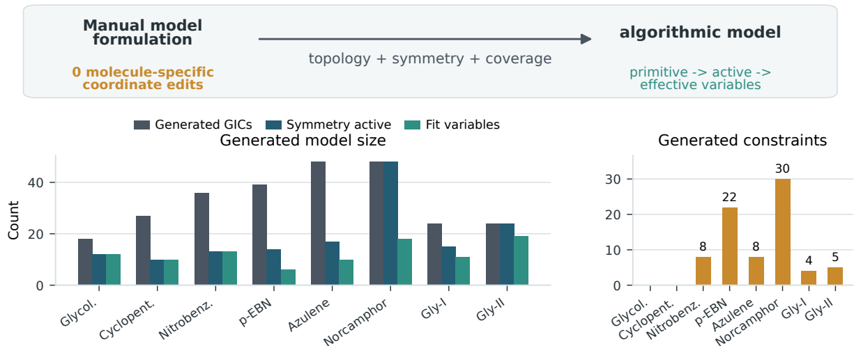
FIG. 3. Model-construction audit for the representative refinements. The top guide links the manual formulation problem to the generated model: topological analysis, symmetry assignment, and isotopic coverage replace molecule-specific coordinate edits under the default global thresholds. The left panel reports the number of generated coordinates, the symmetry-active subset before constraint projection, and the final least-squares variables after reduction. The right panel reports the number of constraints or frozen primitive parameters projected by the model layer. Manual coordinate-model edits are zero for every case; global defaults can be inspected or overridden, but are not tuned separately for the reported molecules. Detailed fit residuals and ranks are collected in the Supporting Information.
