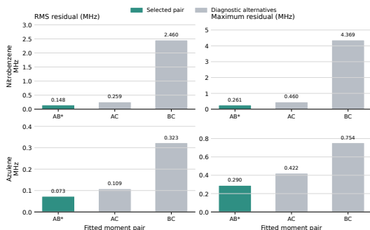
FIG. 4. Planar-component selection for nitrobenzene and azulene: the selected AB pair is highlighted and minimizes the complete post-fit diagnostic residual while the omitted component remains an external check. Detailed values are reported in the Supporting Information.
