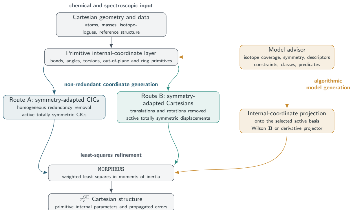
FIG. 1. Architecture of the model-generation framework.
