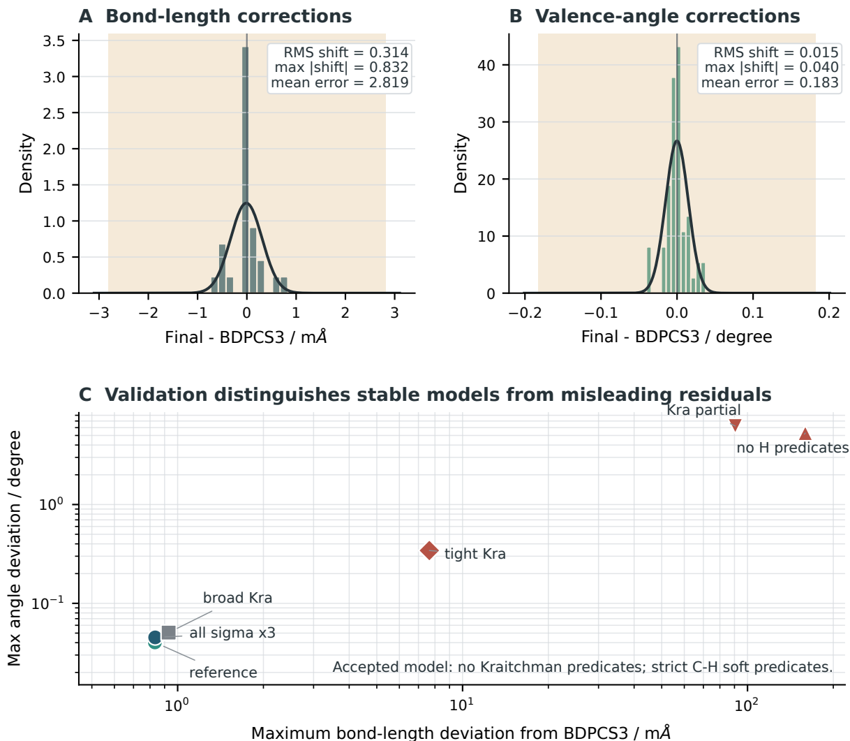
FIG. 8. Camphor validation stress test. Panels A and B show the signed final-minus-BDPCS3 shifts for bond lengths and valence angles in the accepted no-Kraitchman model; the curves are normal distributions fitted to the signed shifts, and the shaded intervals indicate the mean propagated standard error. Panel C compares selected stability variants by the maximum structural deviation from the BDPCS3 reference. The selected model and predicate-width perturbations remain in the sub-milliangstrom, few-hundredths-of-a-degree region, whereas models that remove hydrogen predicates or impose tight Kraitchman-derived predicates can yield superficially acceptable rotational residuals while distorting the geometry.
