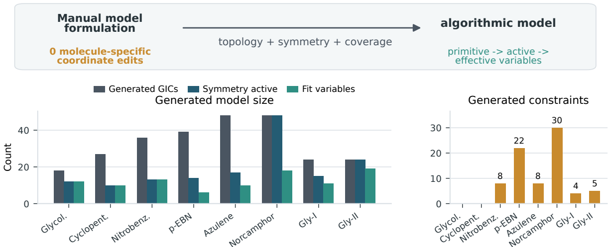
FIG. 4. Model-construction audit for the representative refinements. The top guide links the manual formulation problem to the generated model: topological analysis, symmetry assignment, and isotopic coverage replace molecule-specific coordinate edits under the default global thresholds. The left panel reports the number of generated coordinates, the symmetry-active subset before constraint projection, and the final least-squares variables after reduction. The right panel reports the number of constraints or frozen primitive parameters projected by the model layer. Manual coordinate-model edits are zero for every case; global defaults can be inspected or overridden, but are not tuned separately for the reported molecules. Detailed fit residuals and ranks are collected in the Supporting Information.
