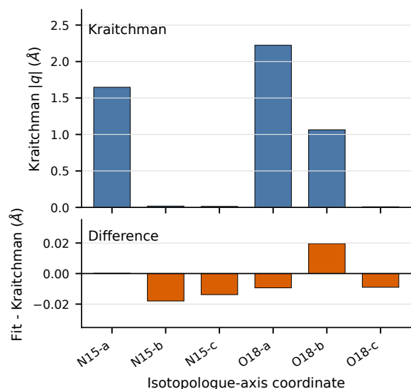
FIG. 6. Kraitchman diagnostic for the nitrobenzene planar benchmark. The upper panel reports absolute substitution coordinates from the Kraitchman analysis. The lower panel reports signed differences between the final SE coordinates and the Kraitchman values on an expanded scale. Numerical values are reported in the Supporting Information.
