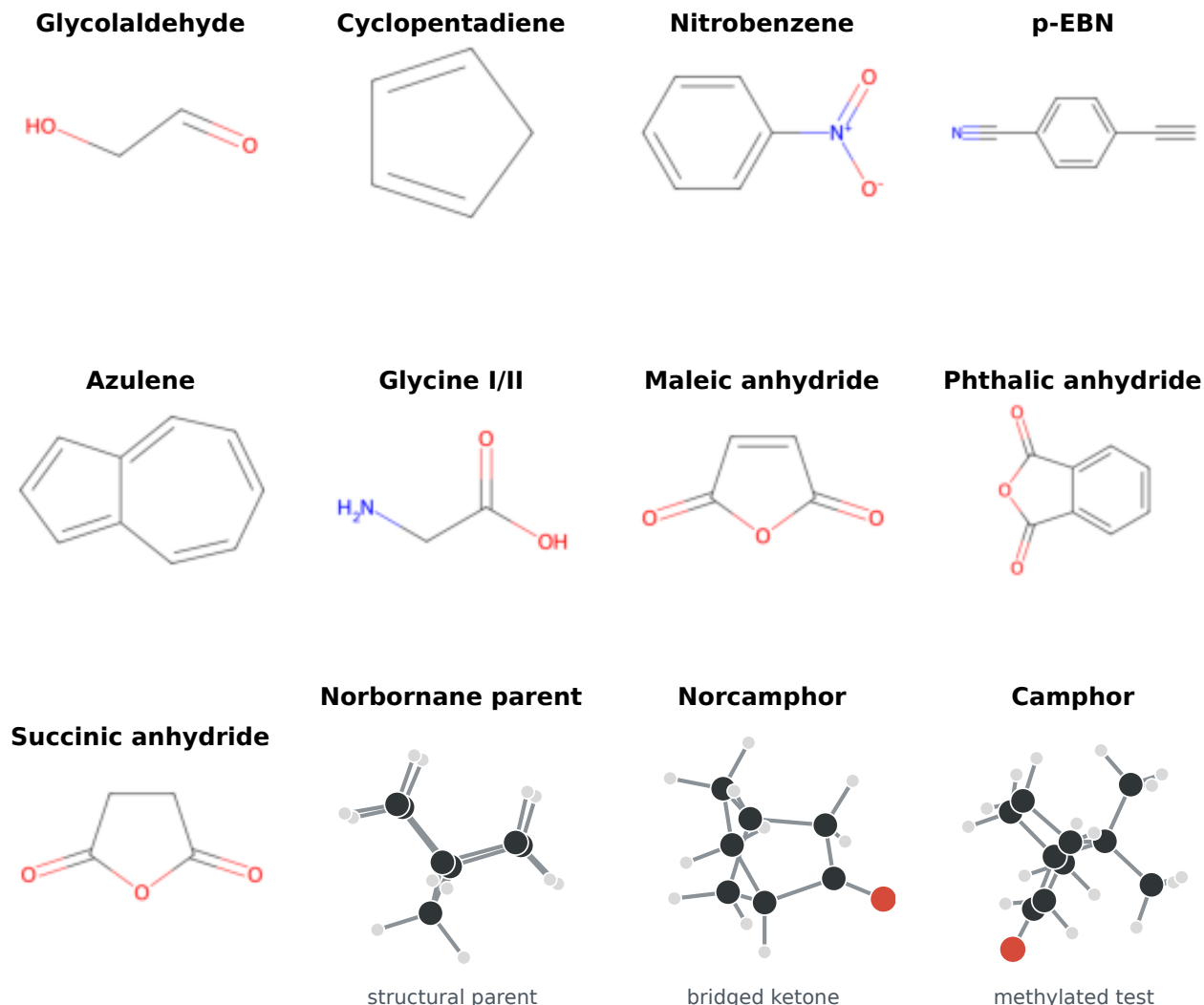
FIG. 3. Molecular structures used to test automated model construction. The acyclic, planar, aromatic, glycine, and anhydride benchmarks are shown as connectivity diagrams; the bridged norbornane family is shown as three-dimensional structures because its graph topology is not communicated adequately by a planar drawing. Norbornane is included as the structural parent of the bridged series, while norcamphor and camphor are the semiexperimental validation cases. Testosterone is shown separately in the large-molecule demonstration. Detailed atom numbering for the tabulated structural parameters is given in the Supporting Information.
