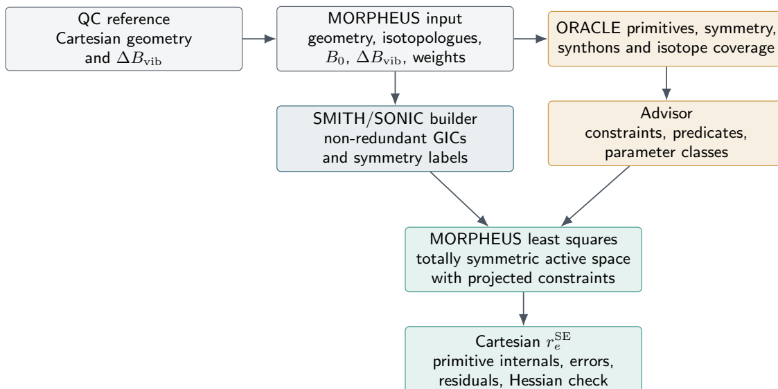
FIG. 9. End-to-end glycine refinement starting from QC Cartesian reference geometries and vibrational corrections. The calculation uses the common job/xyzin container, chemical descriptors, and isotope coverage to generate the active coordinate and constraint model without manually selected fit variables.
