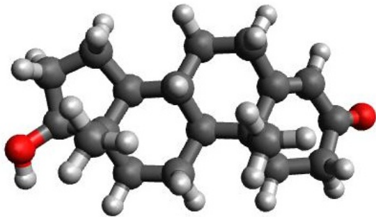
FIG. 10. Testosterone QC geometry used for the large-molecule demonstration.
