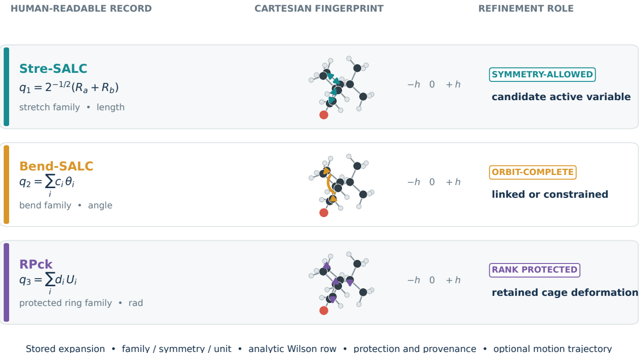
FIG. 2. Inspectable SONIC variables at the MORPHEUS model boundary. Three representative homogeneous families are shown on the reported camphor geometry: the stored record exposes the primitive expansion and units, the Cartesian fingerprint makes the associated motion visually auditable, and the model layer records whether the row is symmetry allowed, linked, constrained, or protected during rank selection. Displacement arrows are enlarged for print; the examples illustrate the traceability contract rather than a finite refinement step.
