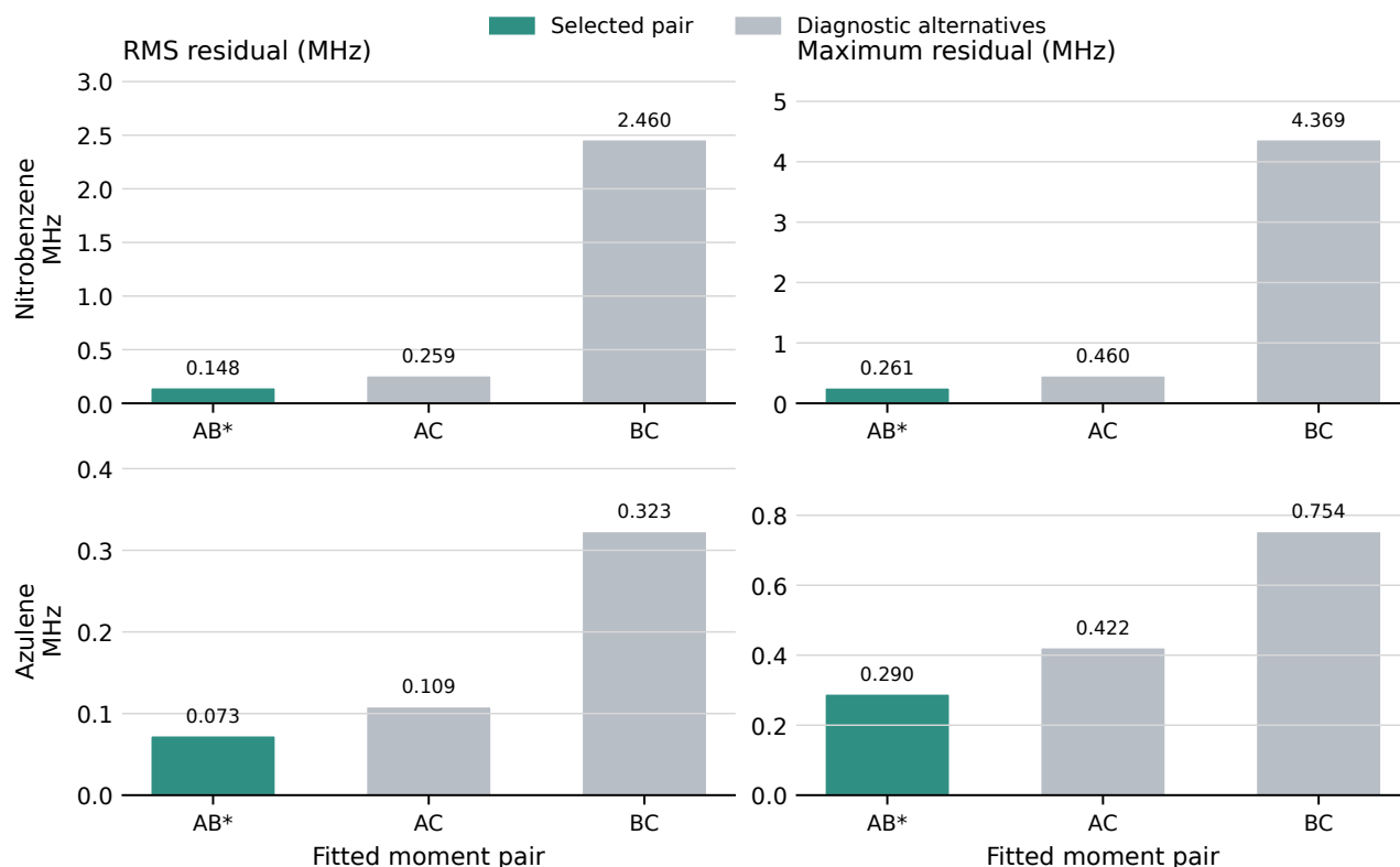
FIG. 5. Planar-component selection for nitrobenzene and azulene: the selected AB pair is highlighted and minimizes the complete post-fit diagnostic residual while the omitted component remains an external check. Detailed values are reported in the Supporting Information.
