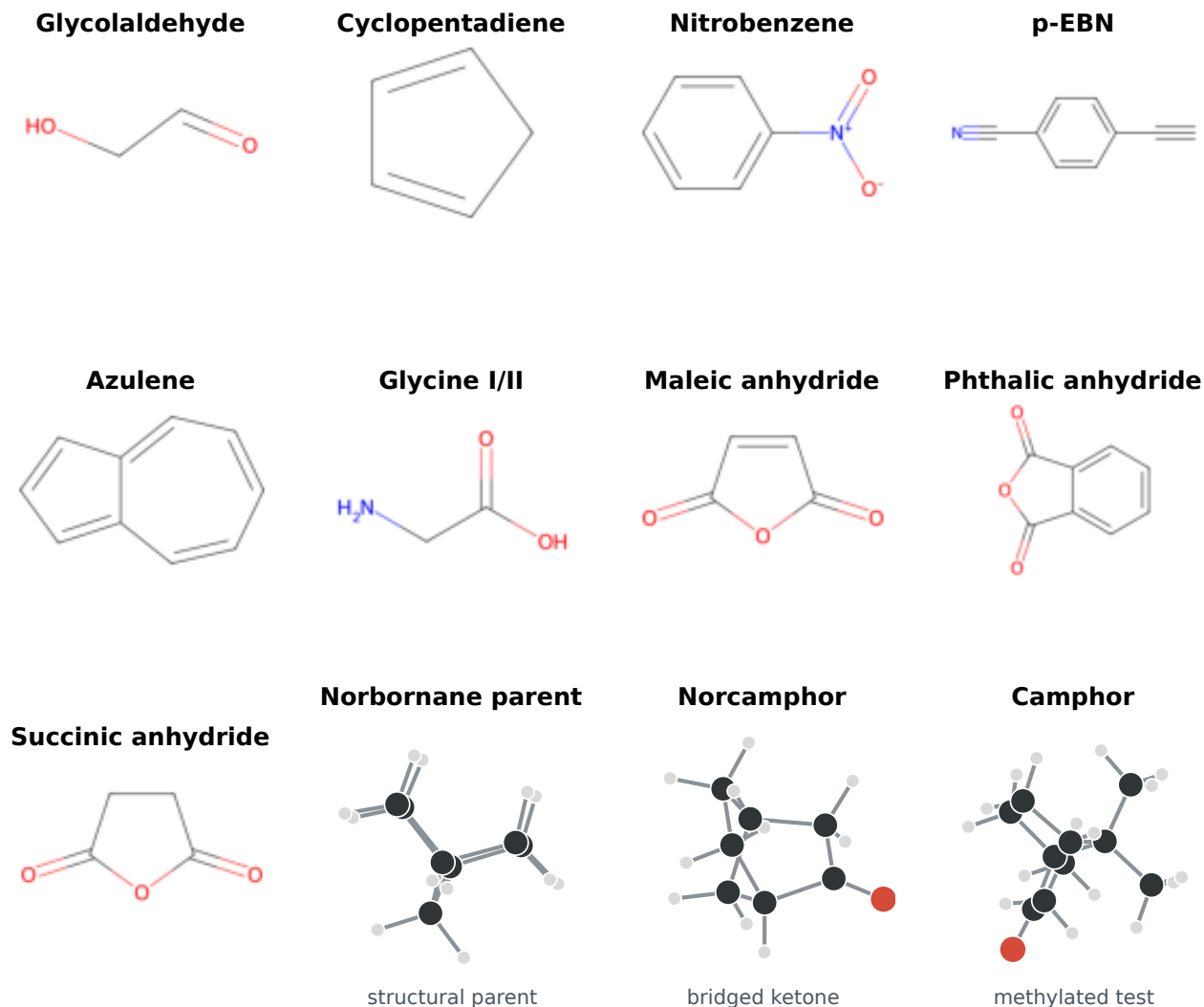
FIG. 3. Molecular structures used to test automated model construction. Connectivity diagrams are used for the acyclic, planar, aromatic, glycine, and anhydride benchmarks; three-dimensional views show the bridged norbornane series. Atom numbering is given in the Supporting Information.
