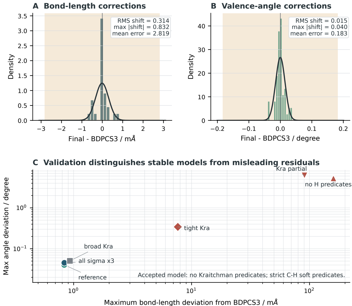
FIG. 8. Camphor validation stress test. Panels A and B give signed bond-length and valence-angle shifts for the accepted model; panel C compares the maximum structural deviations of stability variants.
