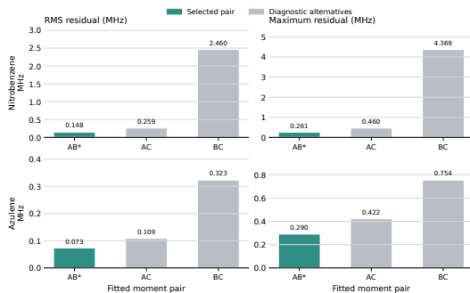
FIG. 5. Planar-component selection for nitrobenzene and azulene. The selected AB pair minimizes the complete diagnostic residual; the omitted component is an external check.
