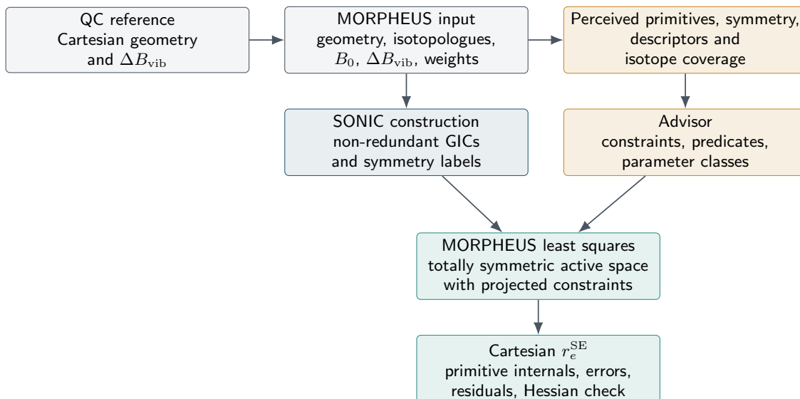
FIG. 9. End-to-end glycine refinement from a quantum-chemical Cartesian reference and vibrational corrections to the generated coordinate and constraint model.
