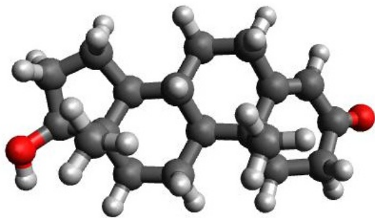
FIG. 10. Testosterone scale demonstration: a 49-atom fused-ring test of automated coordinate generation and reduced structural models.
