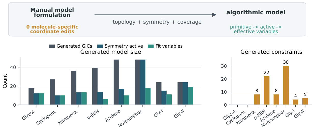
FIG. 4. Model-construction audit for the representative refinements. The left panel gives generated coordinates, the symmetry-active subset, and final fit variables; the right panel gives generated constraints or frozen primitives. All cases use global defaults and no molecule-specific coordinate edits.
