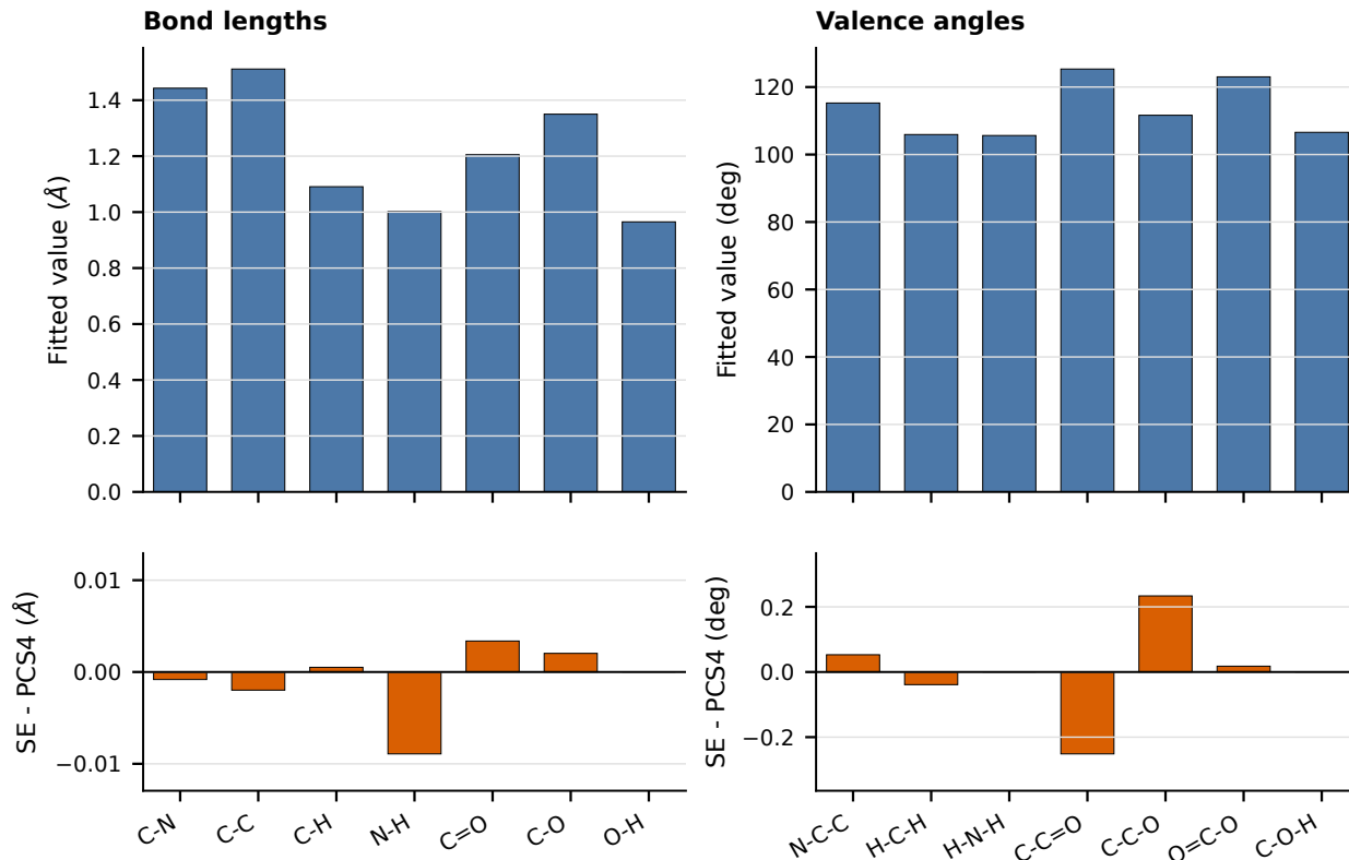
FIG. 7. Glycine I fitted structural parameters and shifts from the QC reference geometry. The upper panels report final SE bond lengths and valence angles; the lower panels report signed SE-QC differences on expanded scales.
