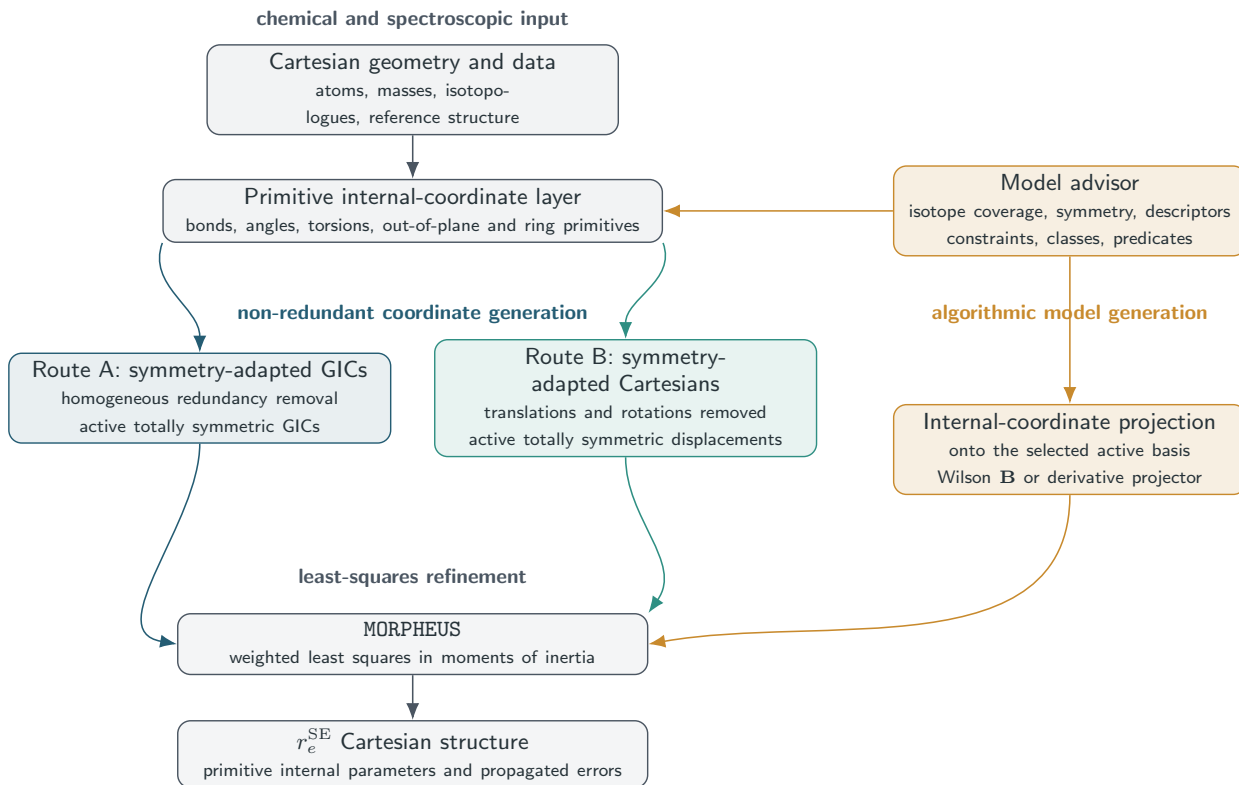
FIG. 1. Architecture of the model-generation framework.
