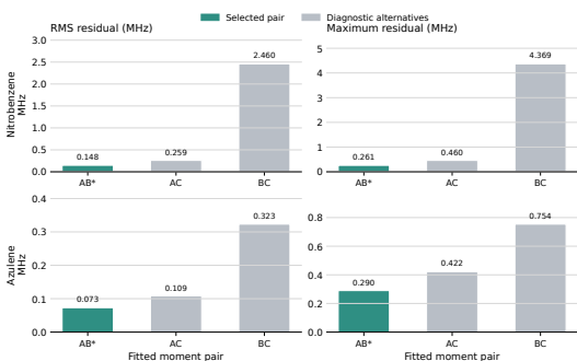
FIG. 5. Planar-component selection for nitrobenzene and azulene: the selected AB pair is highlighted and minimizes the complete post-fit diagnostic residual while the omitted component remains an external check. Detailed values are reported in the Supporting Information.
