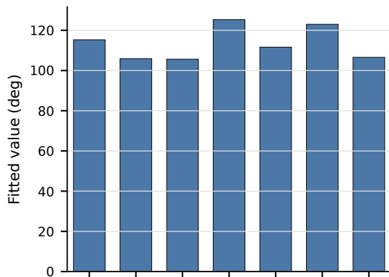
Valence angles
