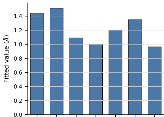
Bond lengths
