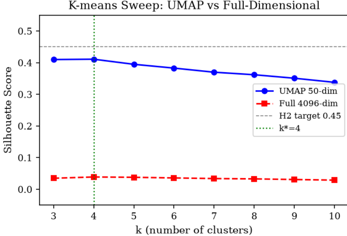
Figure 3: K-means silhouetete sweep. UMAP (blue) achieves S=0.41 at k^*=4 , versus S=0.039 for full 4096-dim embeddings (red dashed). UMAP also reveals a fourth prototype (Privacy) not visible at full dimensionality.
