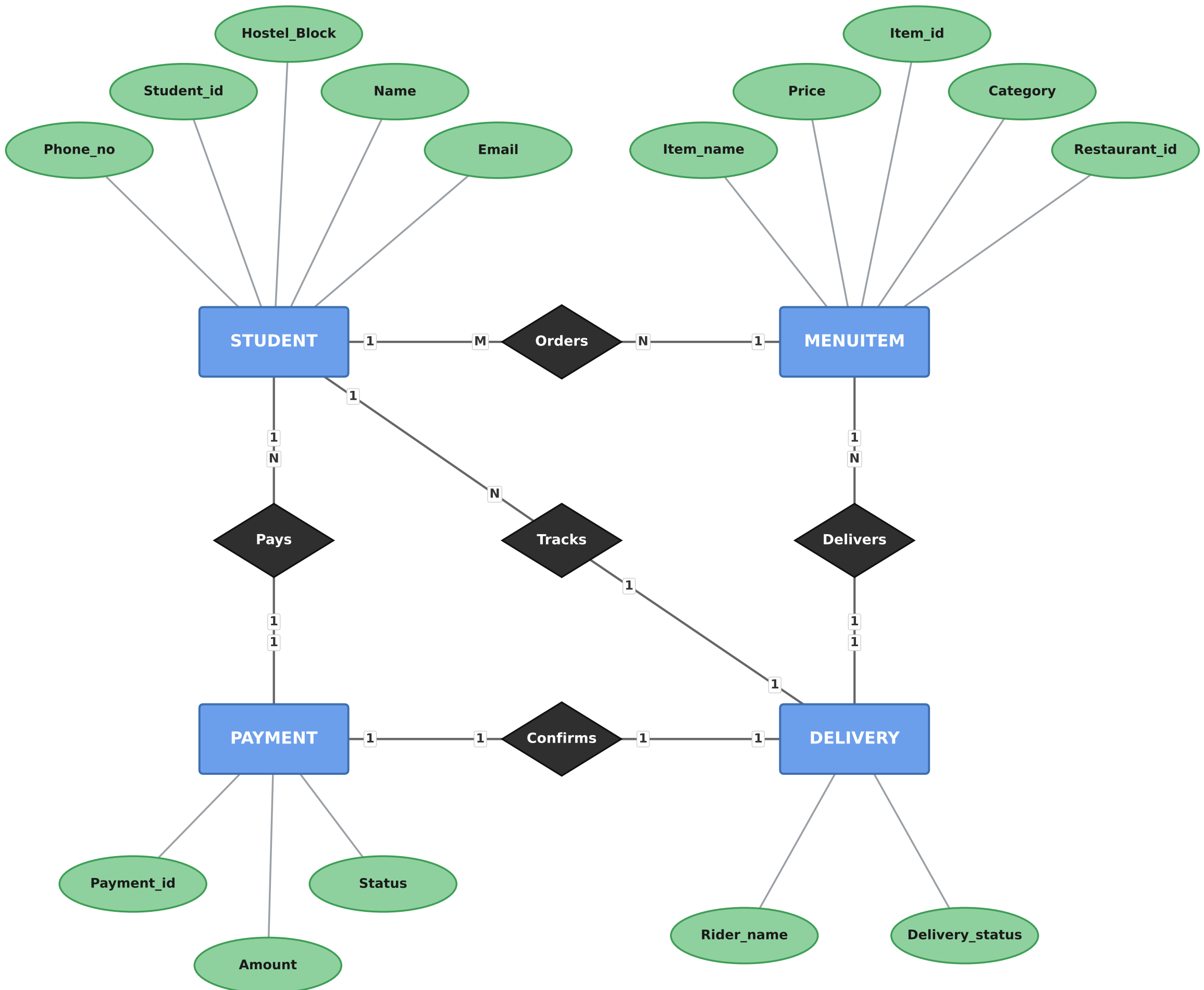
ER DIAGRAM OF CAMPUSEATS
