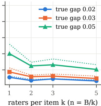
DICES-990, B=900
