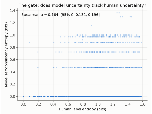
Figure 2: Model self-consistency entropy vs. human label entropy. The model sits at zero entropy on 85% of items regardless of how contested they are; \rho = 0.164 .
