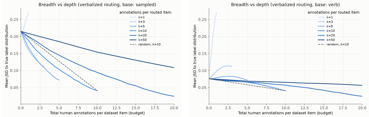
Figure 5: Breadth vs. depth: value of verbalized-entropy routing as a function of total annotation budget, for different annotation depths k per routed item. Left: sampled base — shallow-and-broad ( k = 3-5 ) dominates deep-and-narrow. Right: verbalized base — replacing the model’s verbalized distribution with the empirical distribution of k human labels only breaks even at k \approx 5 ; at k = 1 routing makes the corpus estimate strictly worse.
