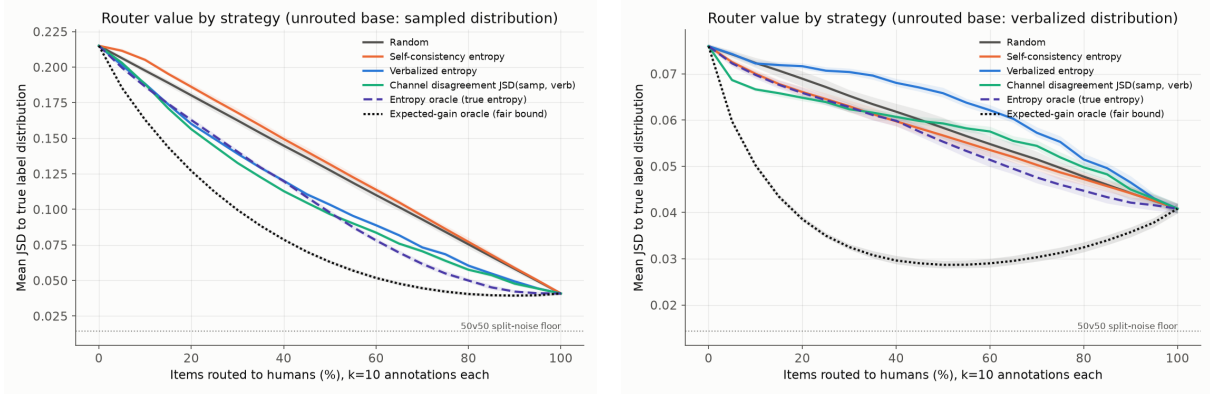
Figure 4: Router value curves at k = 10 annotations per routed item. Left: unrouted items keep the model’s sampled distribution — verbalized-entropy and channel-disagreement routing approach the true-human-entropy oracle. Right: unrouted items keep the model’s verbalized distribution — the same verbalized-entropy signal is now worse than random (anti-selection), and even the true-entropy oracle barely beats random; the expected-gain oracle shows the errors remain findable in principle.
