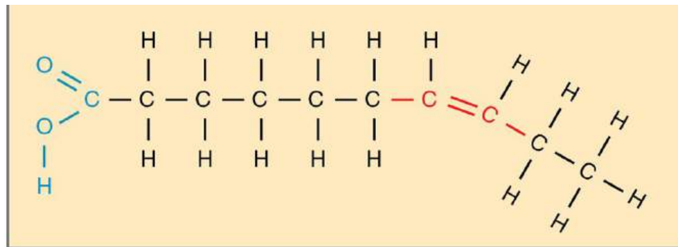
(b) Unsaturated
