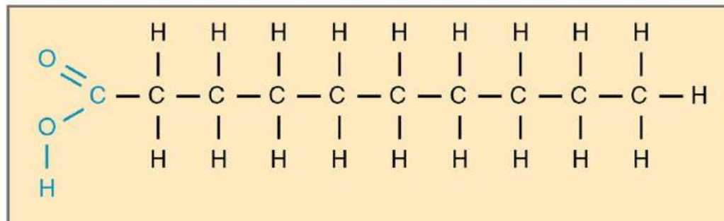
(a) Saturated
