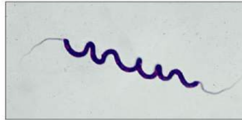
(b) Amphitrichous
