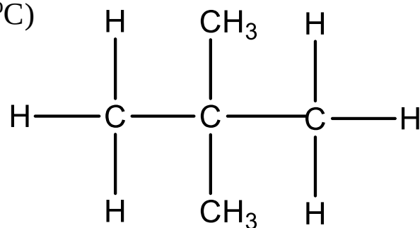
Neopentane
