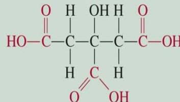
Citric acid
