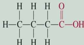
Butyric acid
