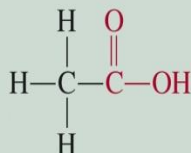
Acetic acid
