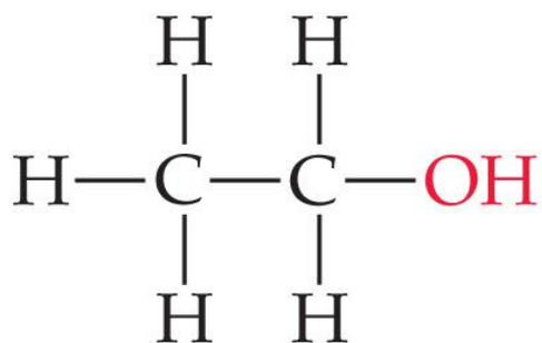
Ethanol
