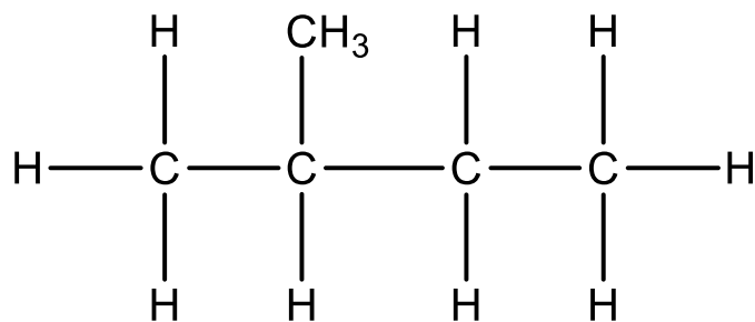
Isopentane
