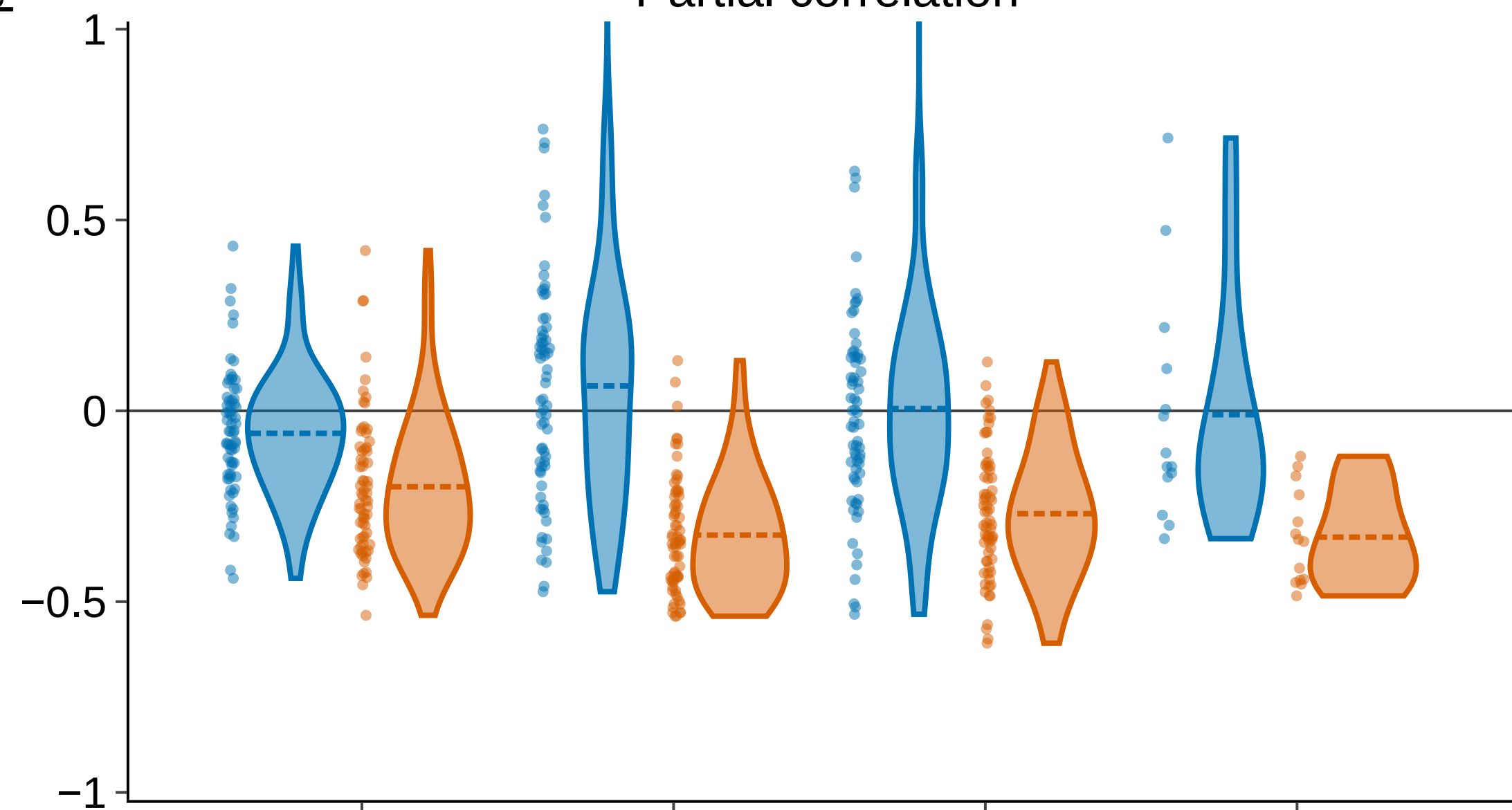
Partial correlation
