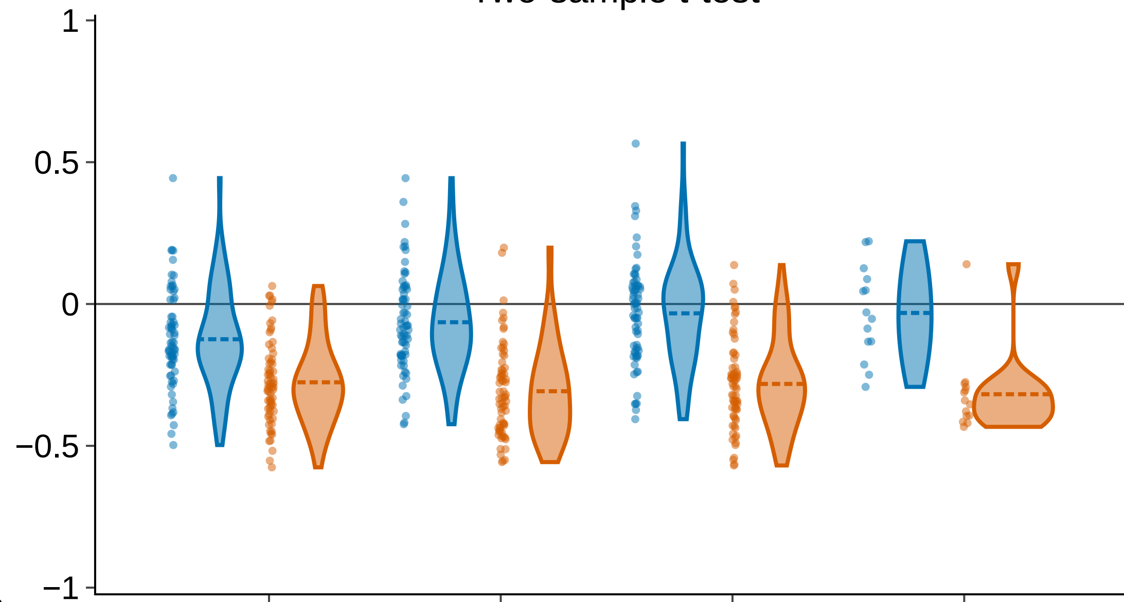
Two-sample t-test
