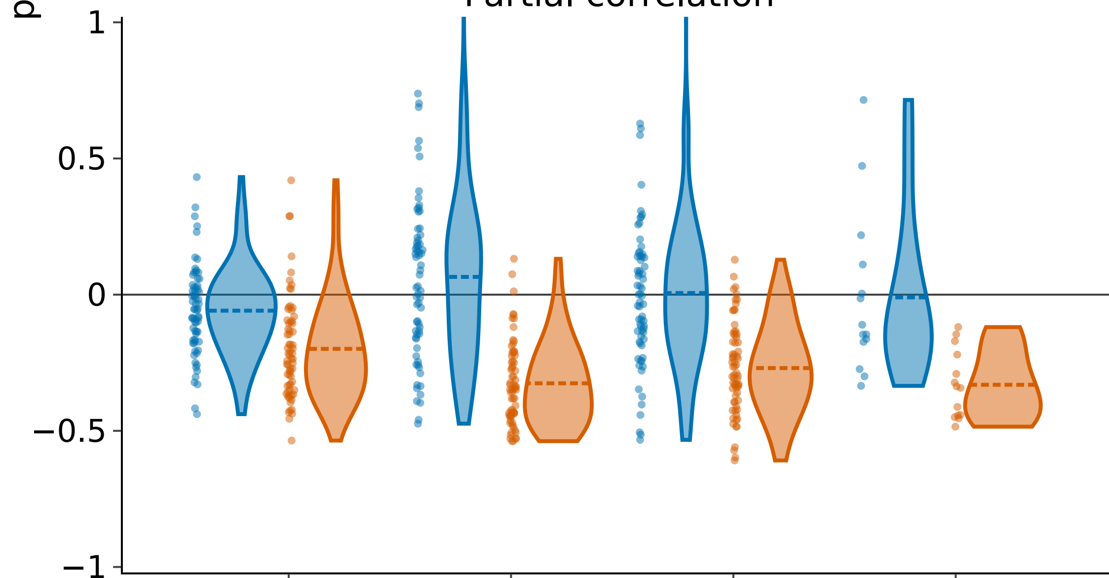
Partial correlation
