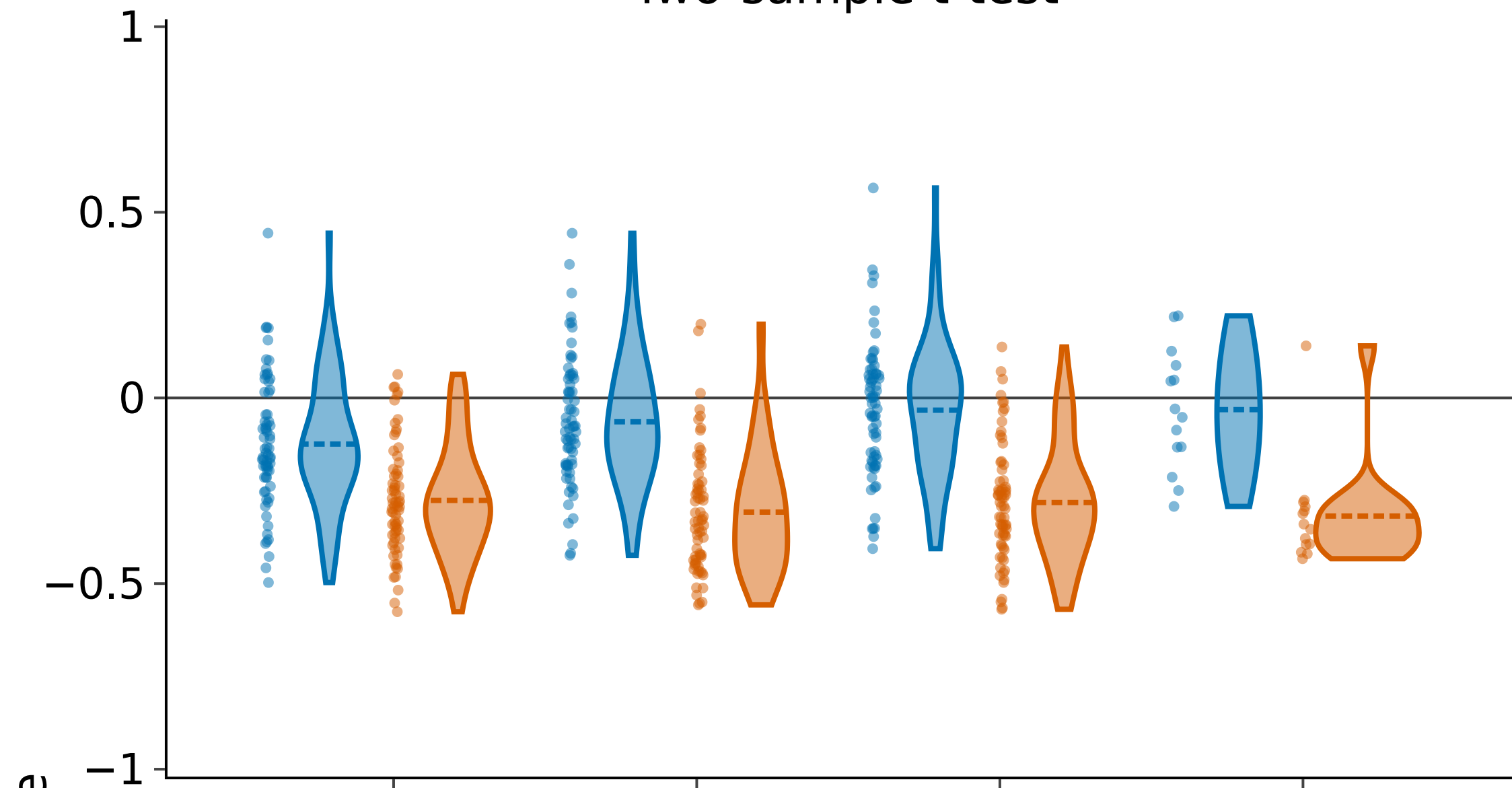
Two-sample t-test
