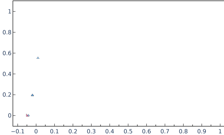
Distance to significance threshold ( p - \alpha )
