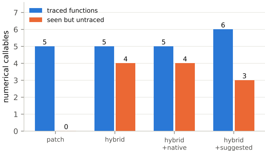
scikit-learn pipeline: observed vs. admitted-unobserved
