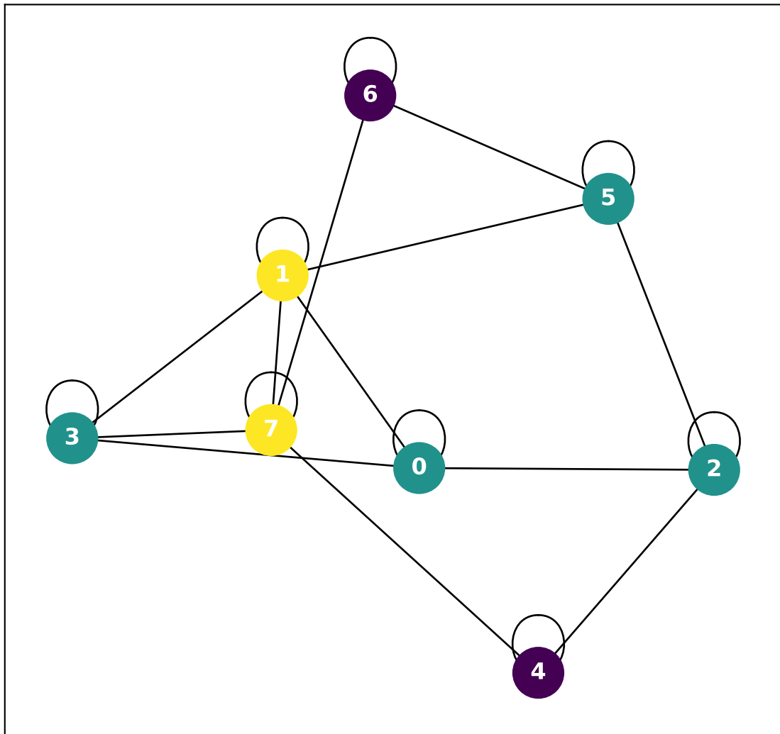
Erdős-Rényi G(8, 0.4) , seed=0
