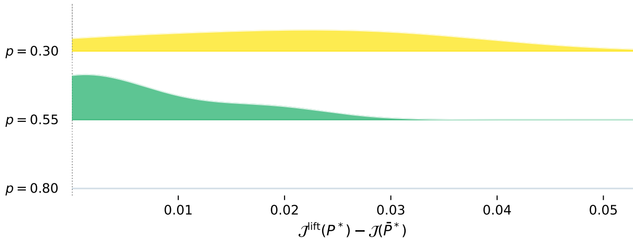
Stackelberg metric improvement via degree lifting, G(6, p)
