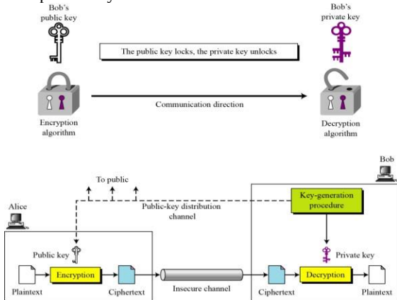
Figure 4.2 Asymmetric-key cryptography
