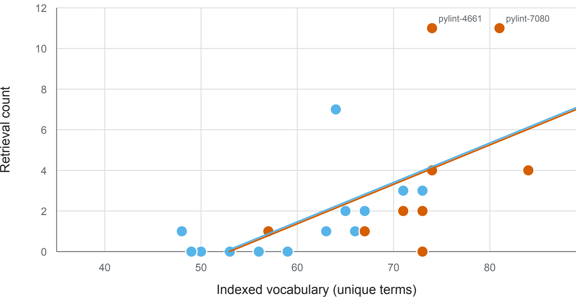
B Indexed vocabulary versus retrieval count
