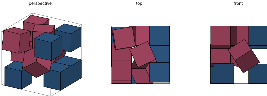
Figure 1: Twelve unit cubes in a cube of side 2.931515. Blue: tilt below 1.5^\circ ; red: tilted.
