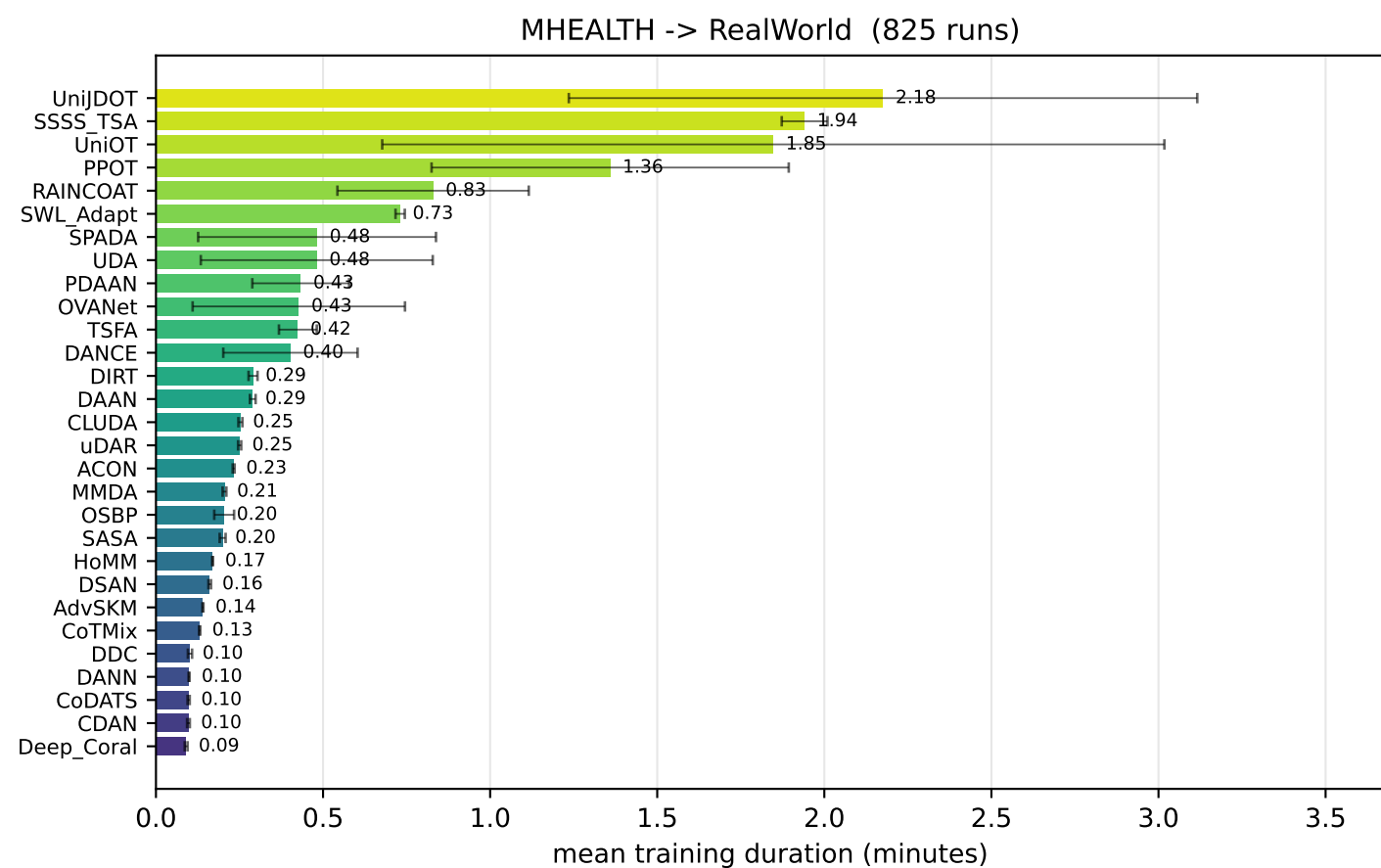
Mean training duration per algorithm — one panel per pair (averaged across scenarios, n_unknown, seeds)
