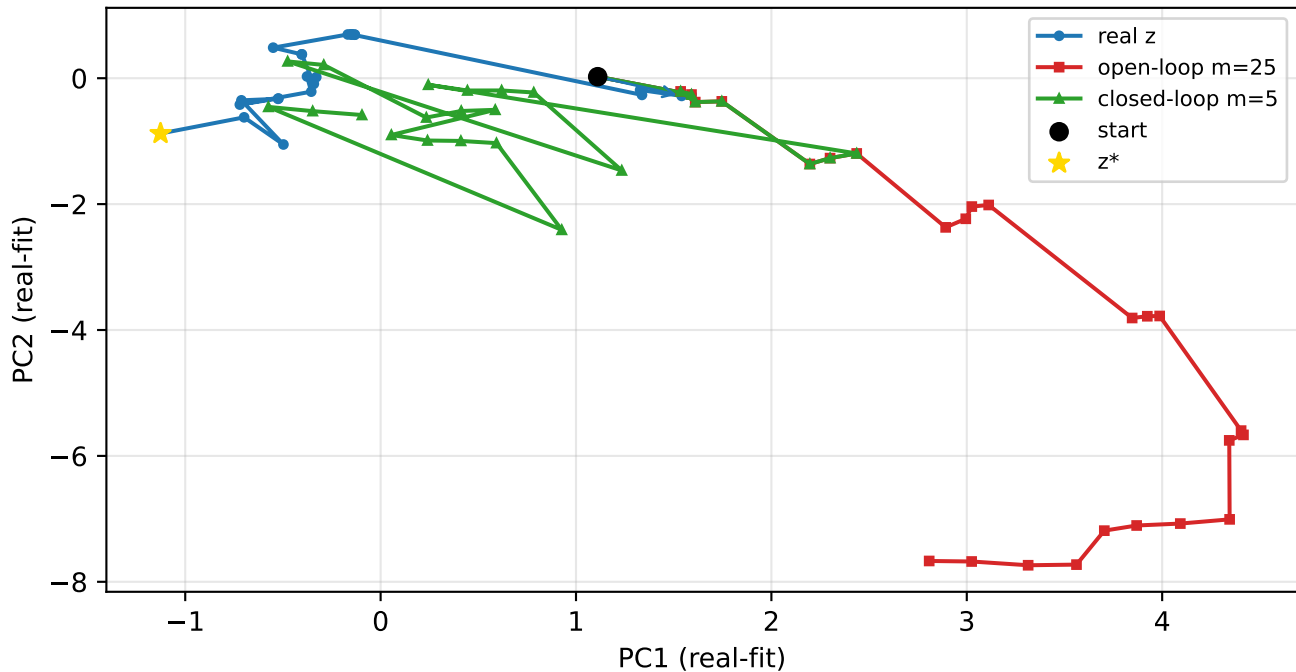
Fig-1 pair 0: PCA captured 81.9% | \|\hat{z}_{\text{end}} - z^*\| m=25=18.84 m=5=2.57 d_start=2.63
