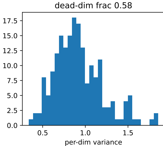
Fig-7 rank dim=192 PR=22.5 elbow90=29 dead=0.58
