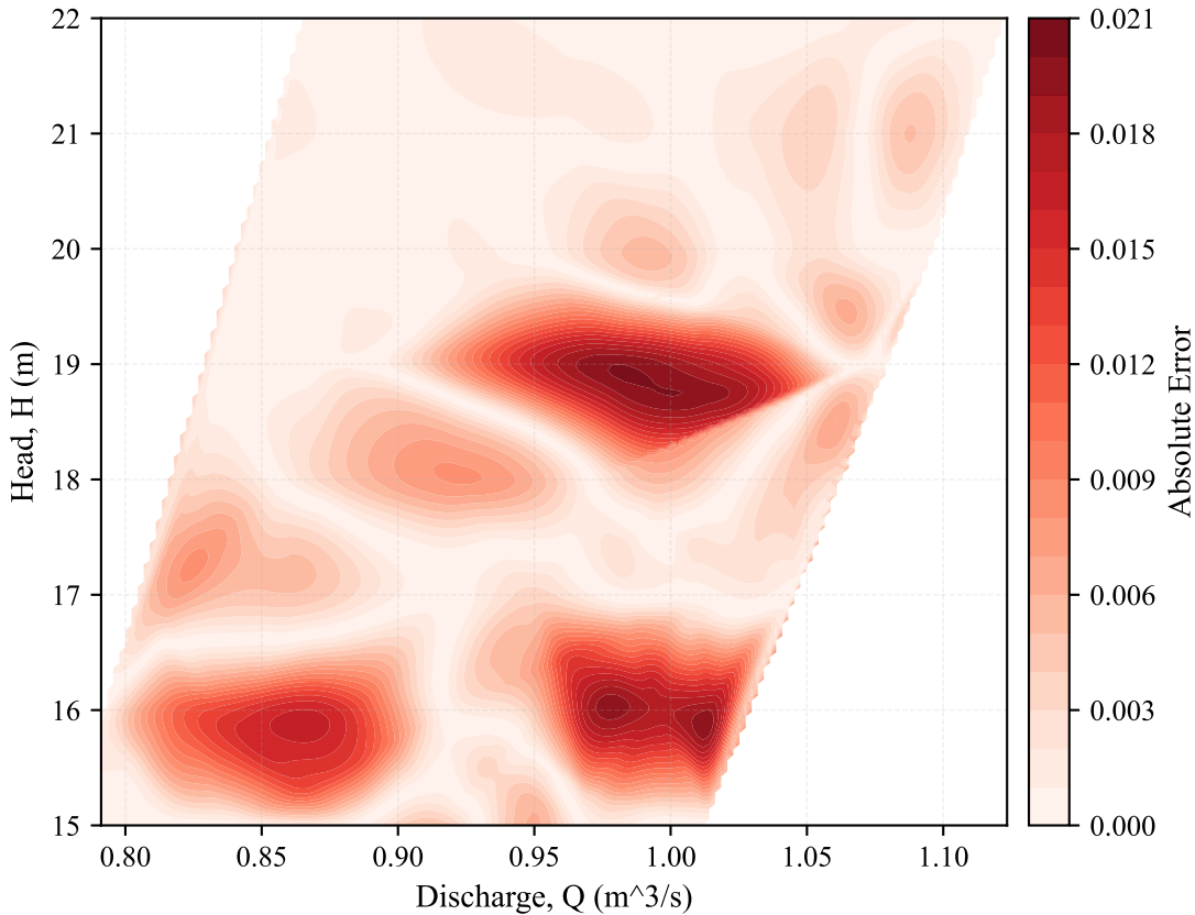
Abs. Error: Ground Truth vs Golden Ratio (Fibonacci) (Mean: 0.0041)
