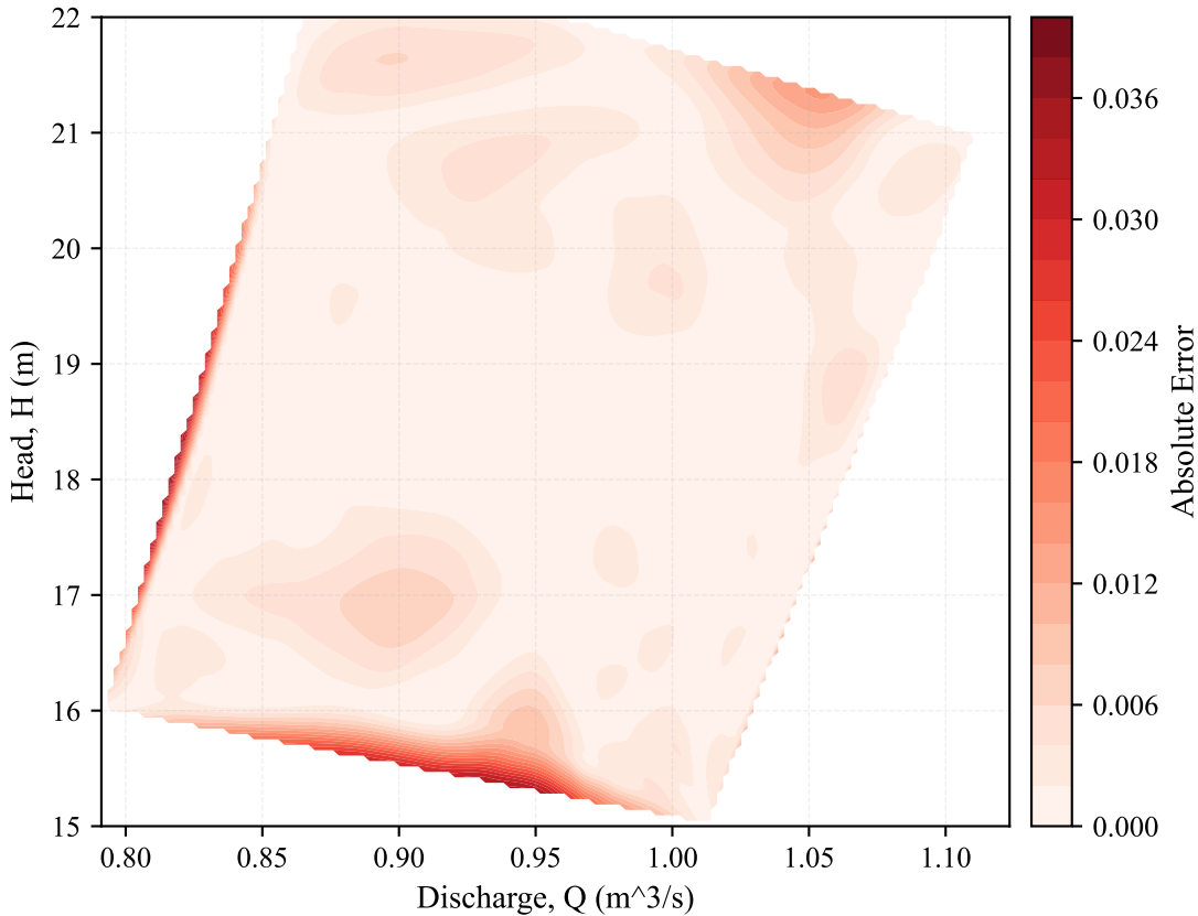
Abs. Error: Ground Truth vs LHS (Mean: 0.0028)
