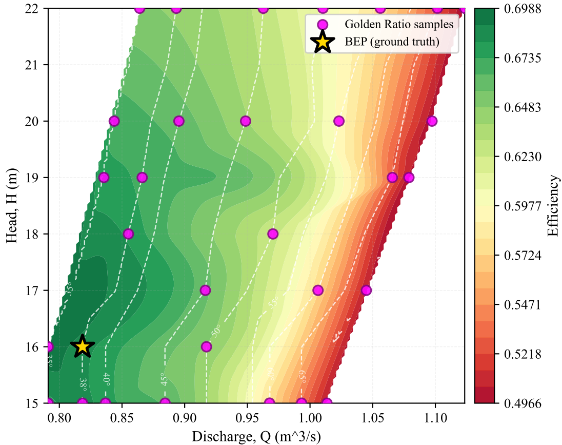
Golden Ratio Prediction (30 exp)
