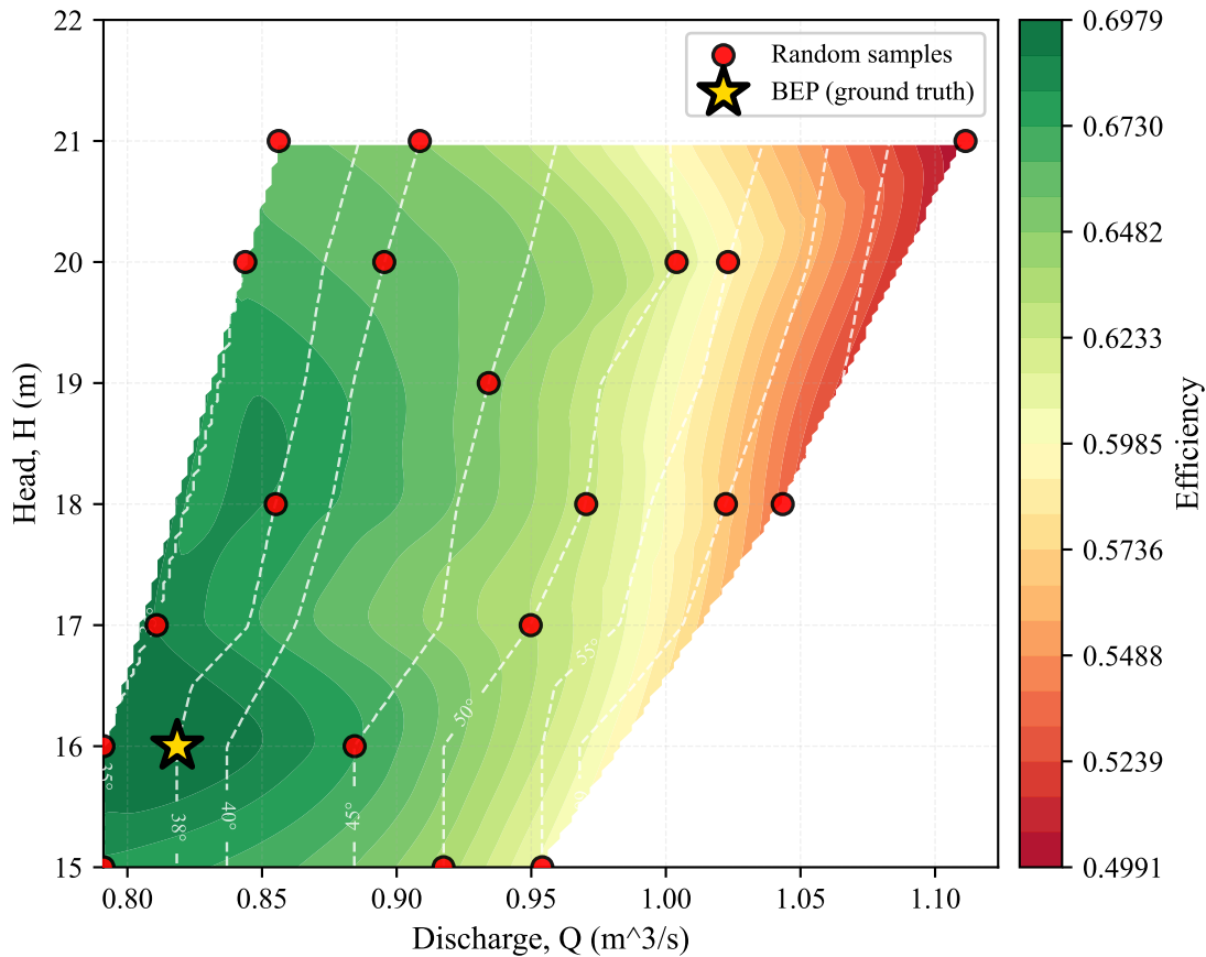
Random Prediction (20 exp)
