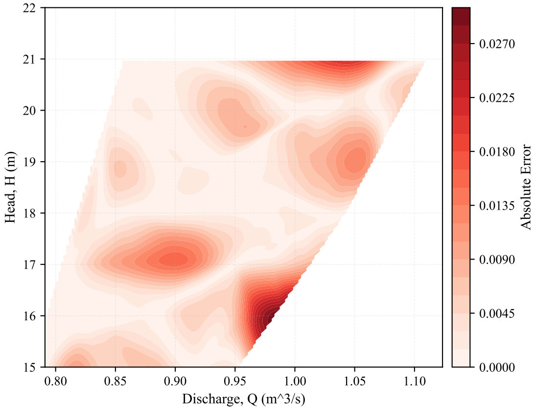
Abs. Error: Ground Truth vs Random (Mean: 0.0044)
