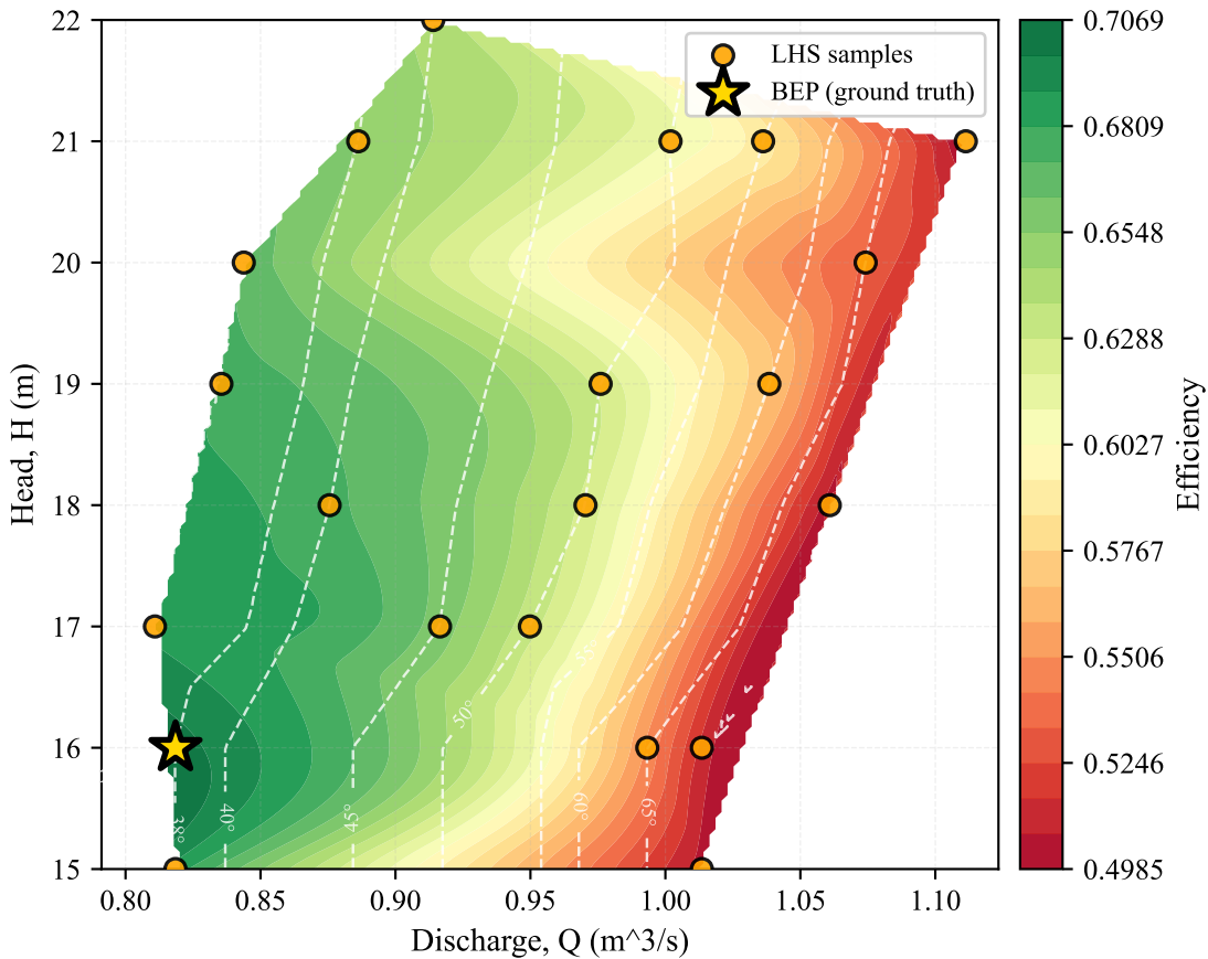
LHS Prediction (20 exp)
