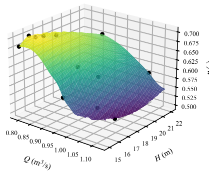
BO-UCB
