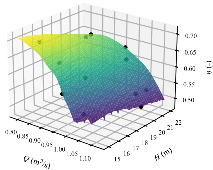
Random
