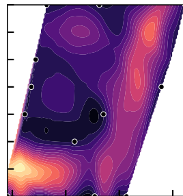
BO-UCB
