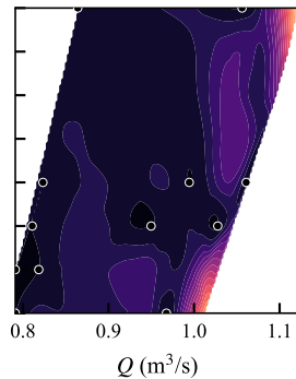
BO-UCB
