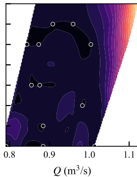
Random
