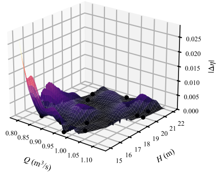
Random
