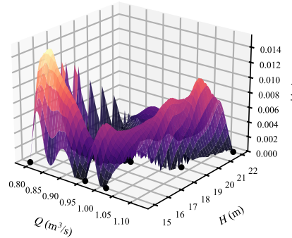
BO-UCB
