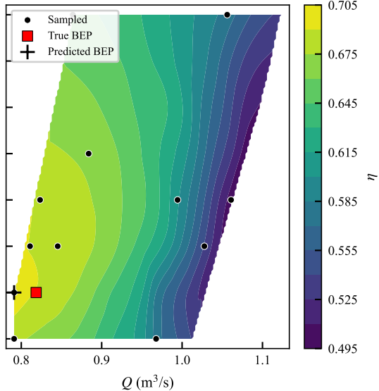
BO-UCB (MAE=0.0056)
