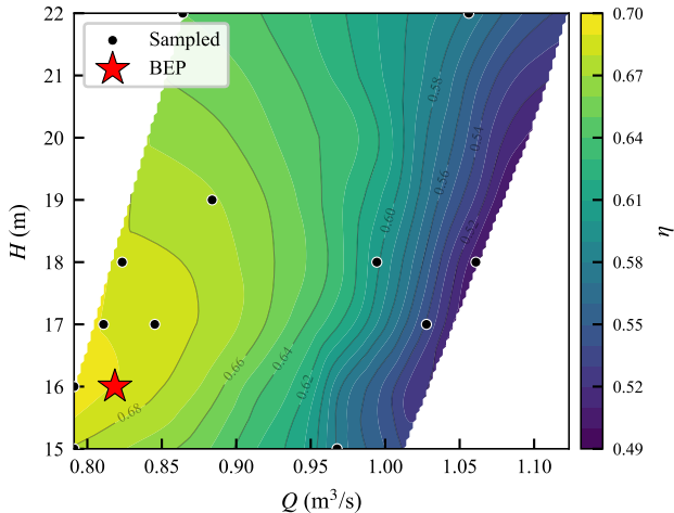
BO-UCB reconstruction ( n = 12 )
