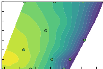
ALM ( n=12 )
