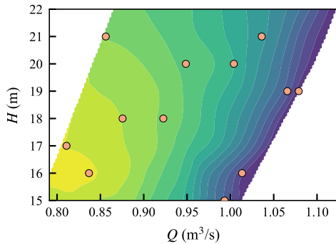
LHS ( n=12 )
