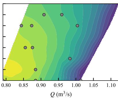
Random ( n=12 )
