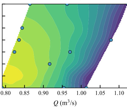
Grid ( n=12 )
