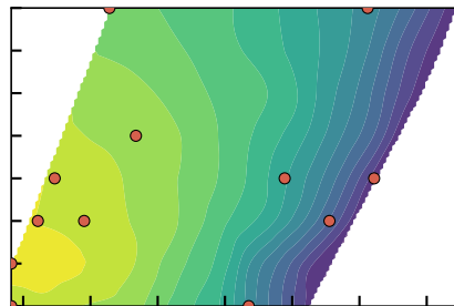
BO-UCB ( n=12 )
