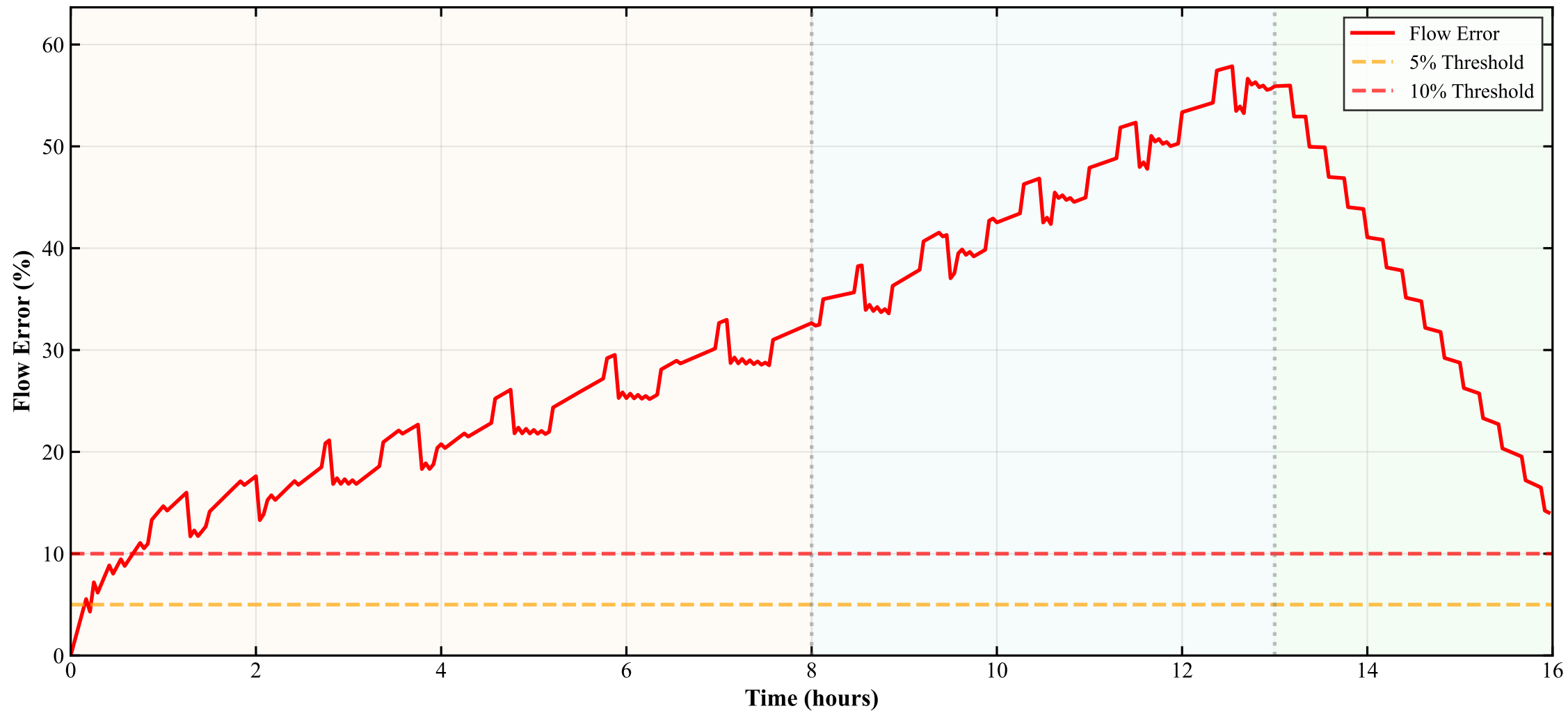
ESC Tracking Error Over Time
