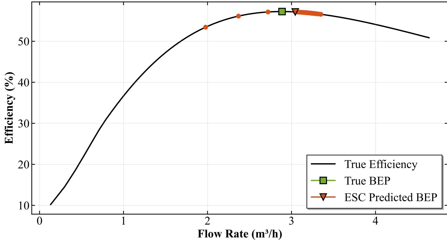
True vs Predicted Efficiency Curve (H = 25.0m)
