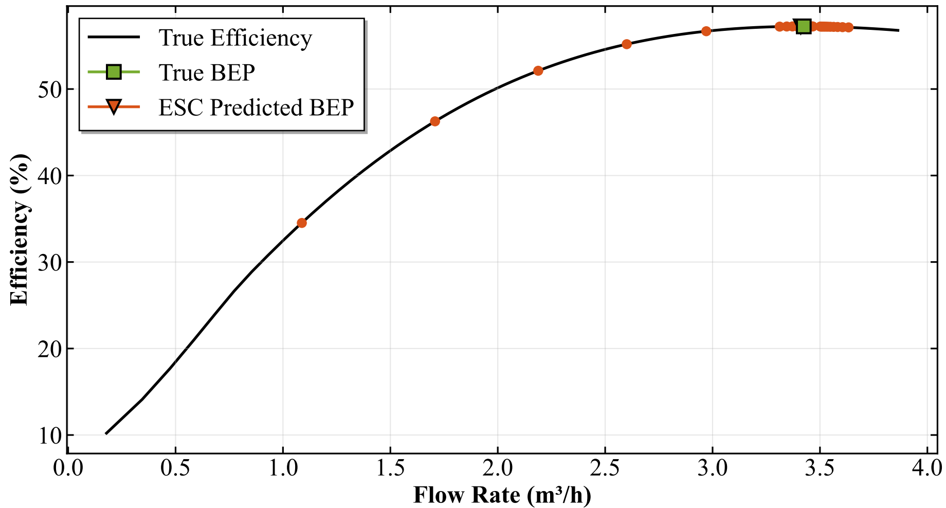
True vs Predicted Efficiency Curve (H = 35.0m)
